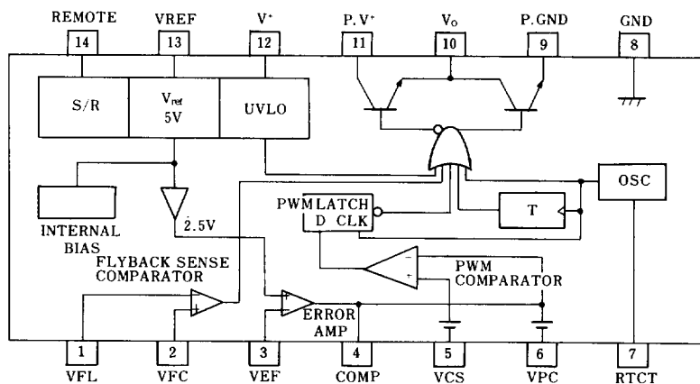
NJM2362D
