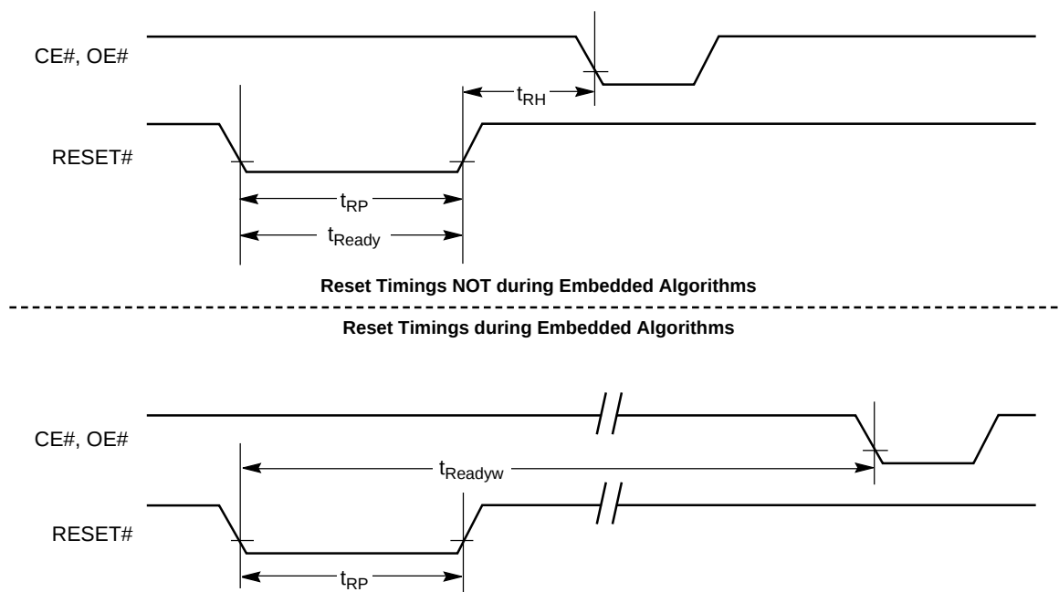
Figure 12. Reset Timings
