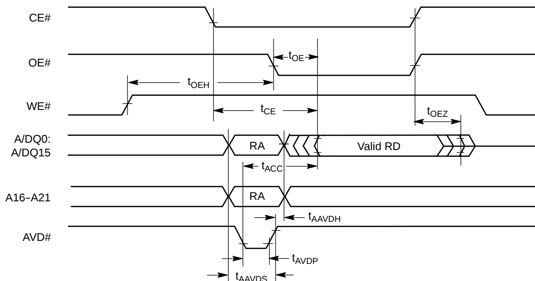
Figure 11. Asynchronous Mode Read
