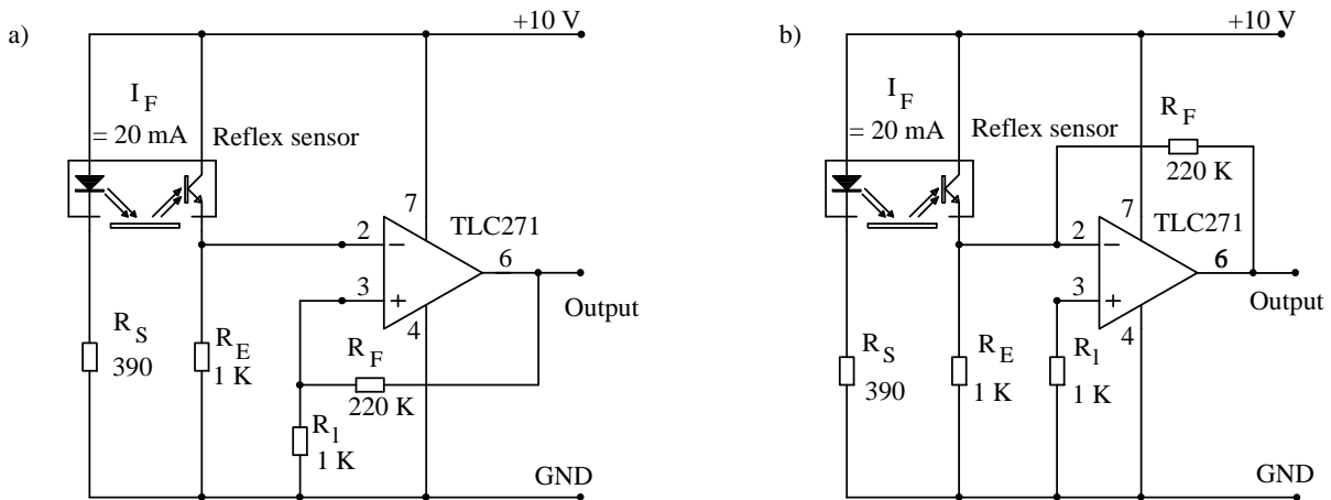
Figure 12 Circuits with operational amplifier
