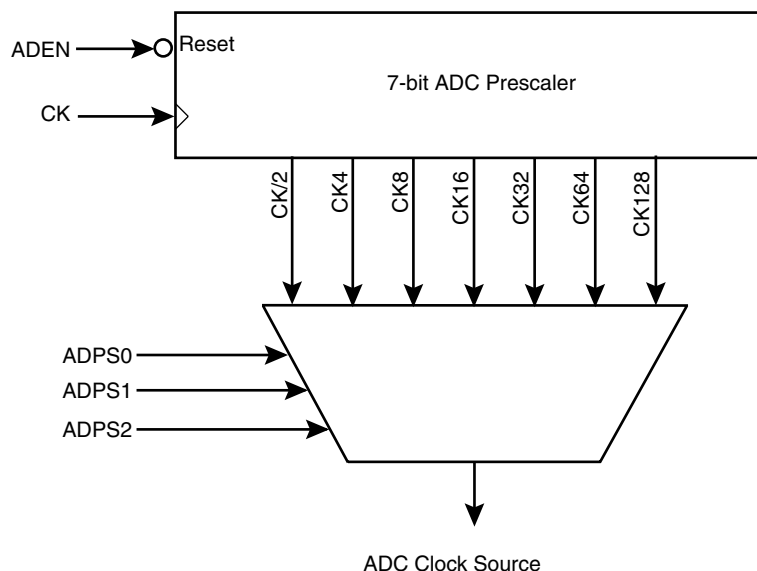
Figure 23. ADC Prescaler
