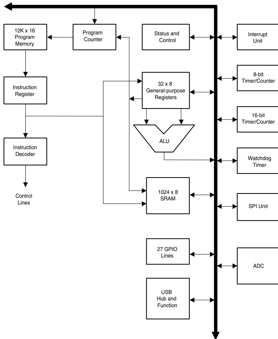
Figure 3. The AT43USB355 Enhanced RISC Architecture
