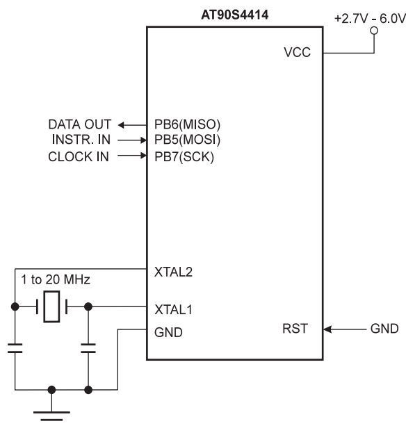
Figure 66. Serial Programming and Verify
