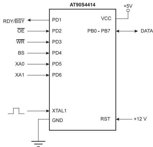
Figure 62. Parallel Programming
