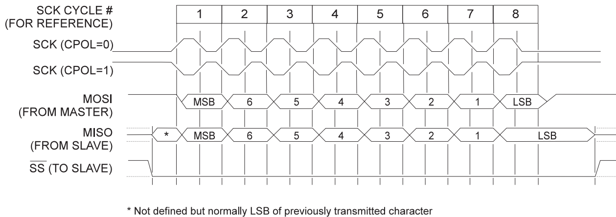
Figure 42. SPI Transfer Format with CPHA = 1
