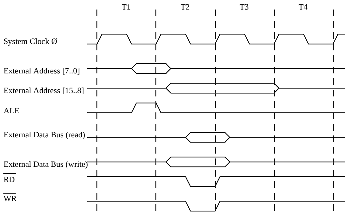
Figure 25. External Data SRAM Memory Cycles with Wait State
