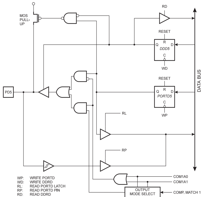
Figure 59. PORTD Schematic Diagram (Pin PD5)
