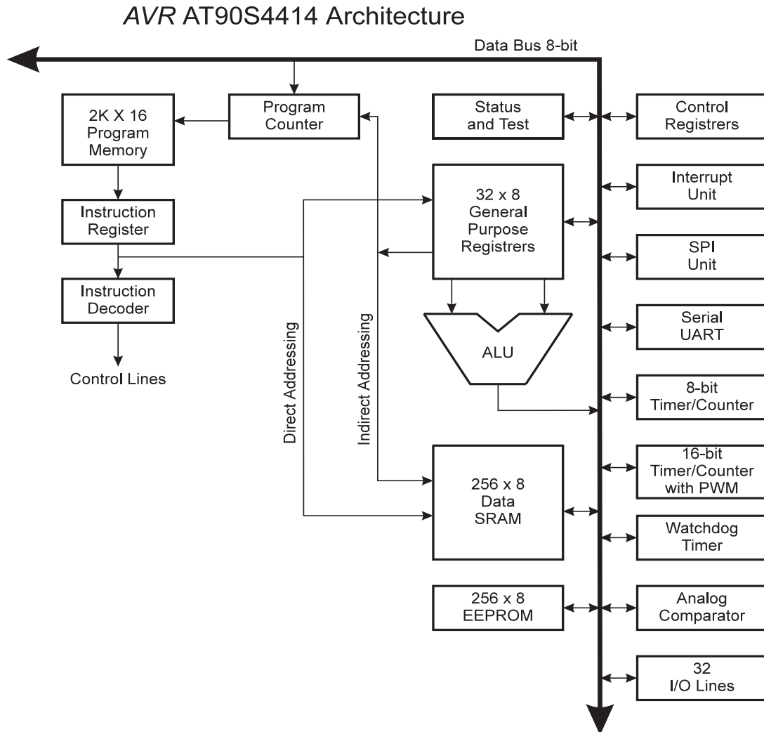
Figure 4. The AT90S4414 AVR Enhanced RISC Architecture
