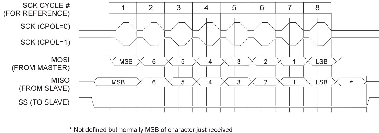
Figure 41. SPI Transfer Format with CPHA = 0
