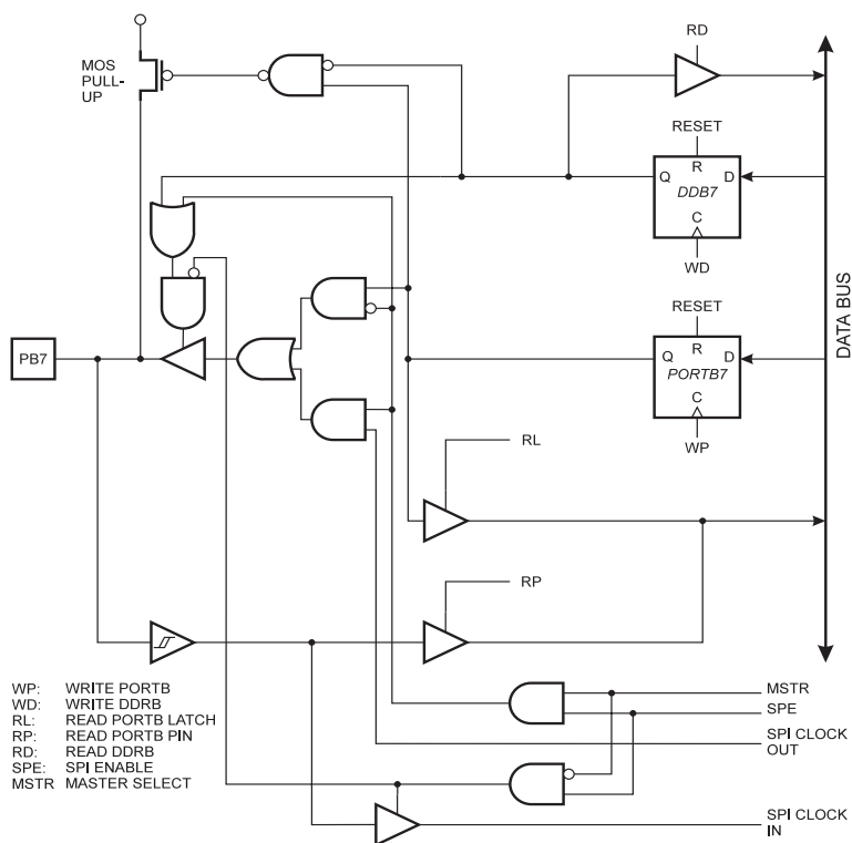
Figure 53. PORTB Schematic Diagram (Pin PB7)
