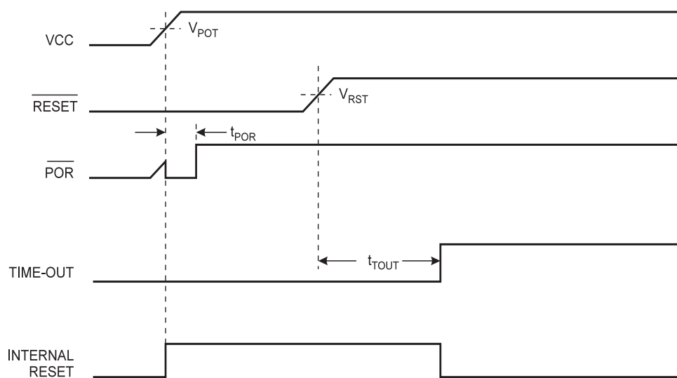
Figure 29. MCU Start-Up, \overline{\text{RESET}} Controlled Externally
