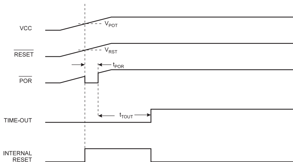
Figure 28. MCU Start-Up, \overline{\text{RESET}} Tied to V_{CC} or Unconnected. Slowly Rising V_{CC}
