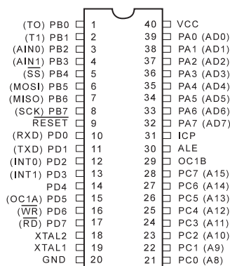
PDIP
