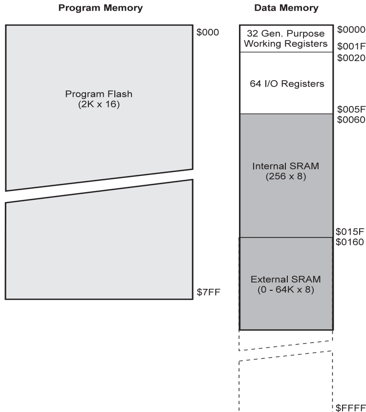
Figure 5. Memory Maps
