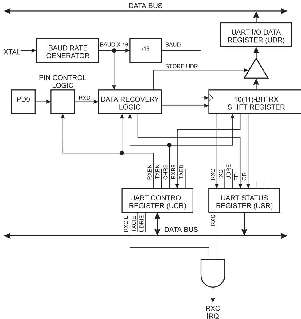
Figure 44. UART Receiver
