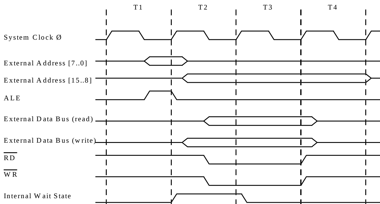
Figure 24. External Data SRAM Memory Cycles without Wait State
