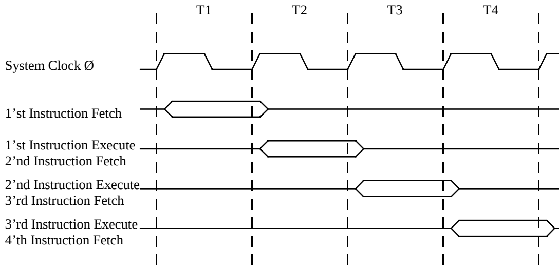
Figure 21. The Parallel Instruction Fetches and Instruction Executions
