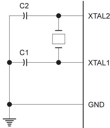
Figure 2. Oscillator Connections
