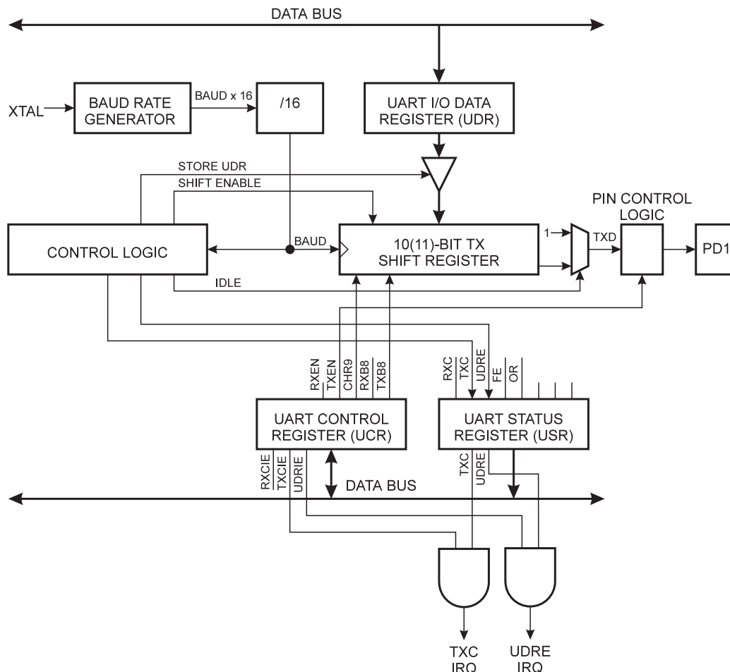
Figure 43. UART Transmitter
