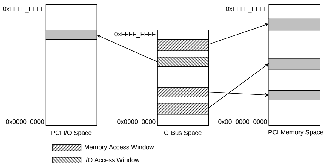
Figure 10.3.3 Initiator Access Memory Window
