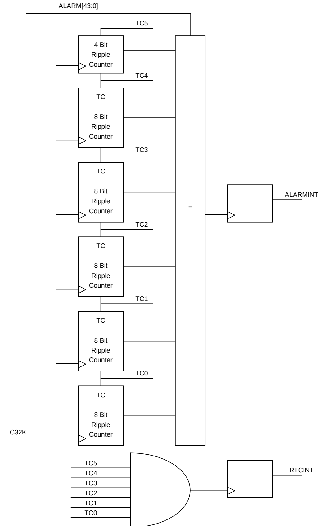
Figure 19.2.1 RTC Block Diagram
