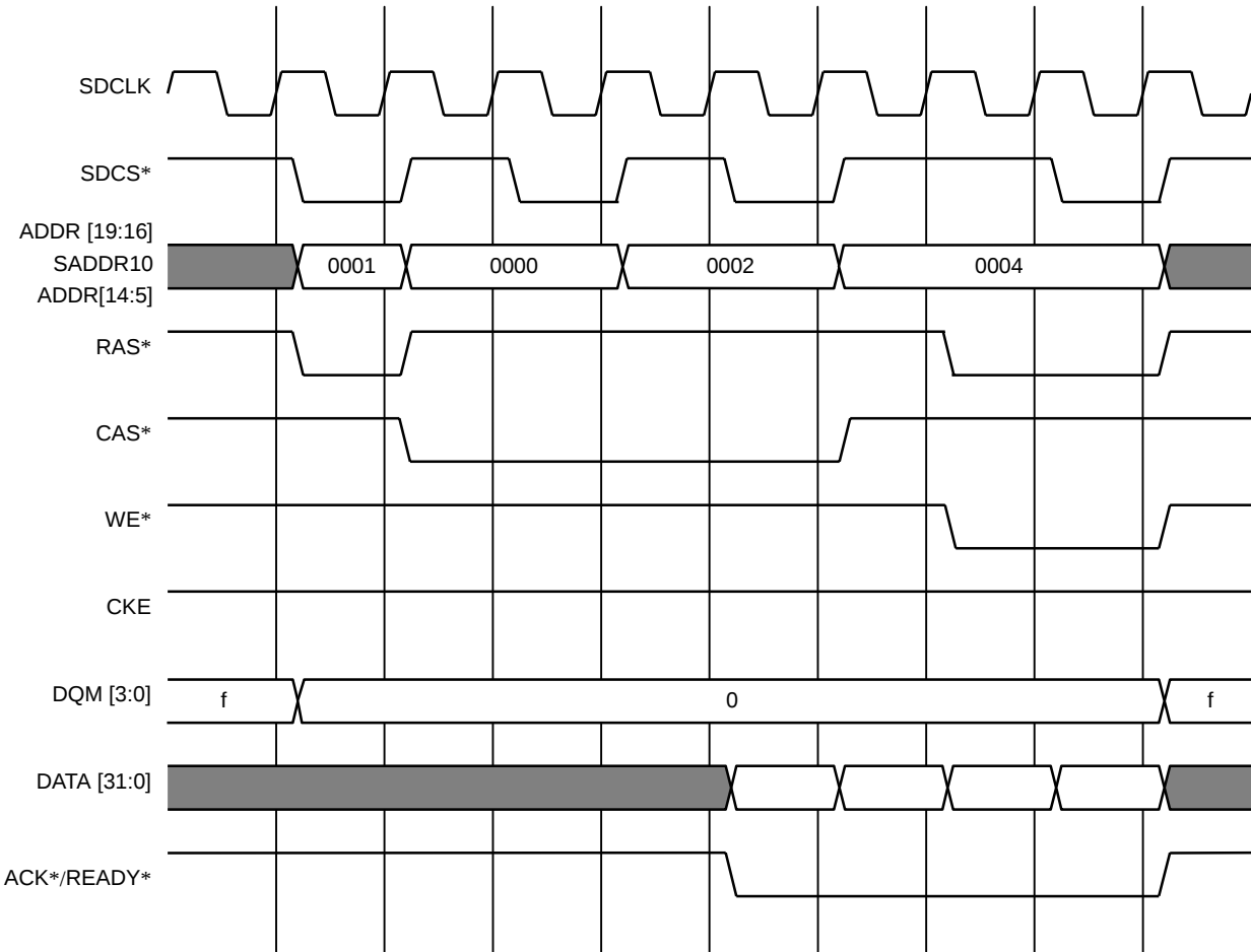
Figure 9.5.5 Four-Word Burst Read ( t_{RCD} = 2 , t_{CASL} = 2 , t_{DA} = 0 , 32-bit Bus)
