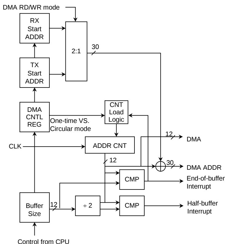
Figure 16.3.3 CHI DMA Address Generation
