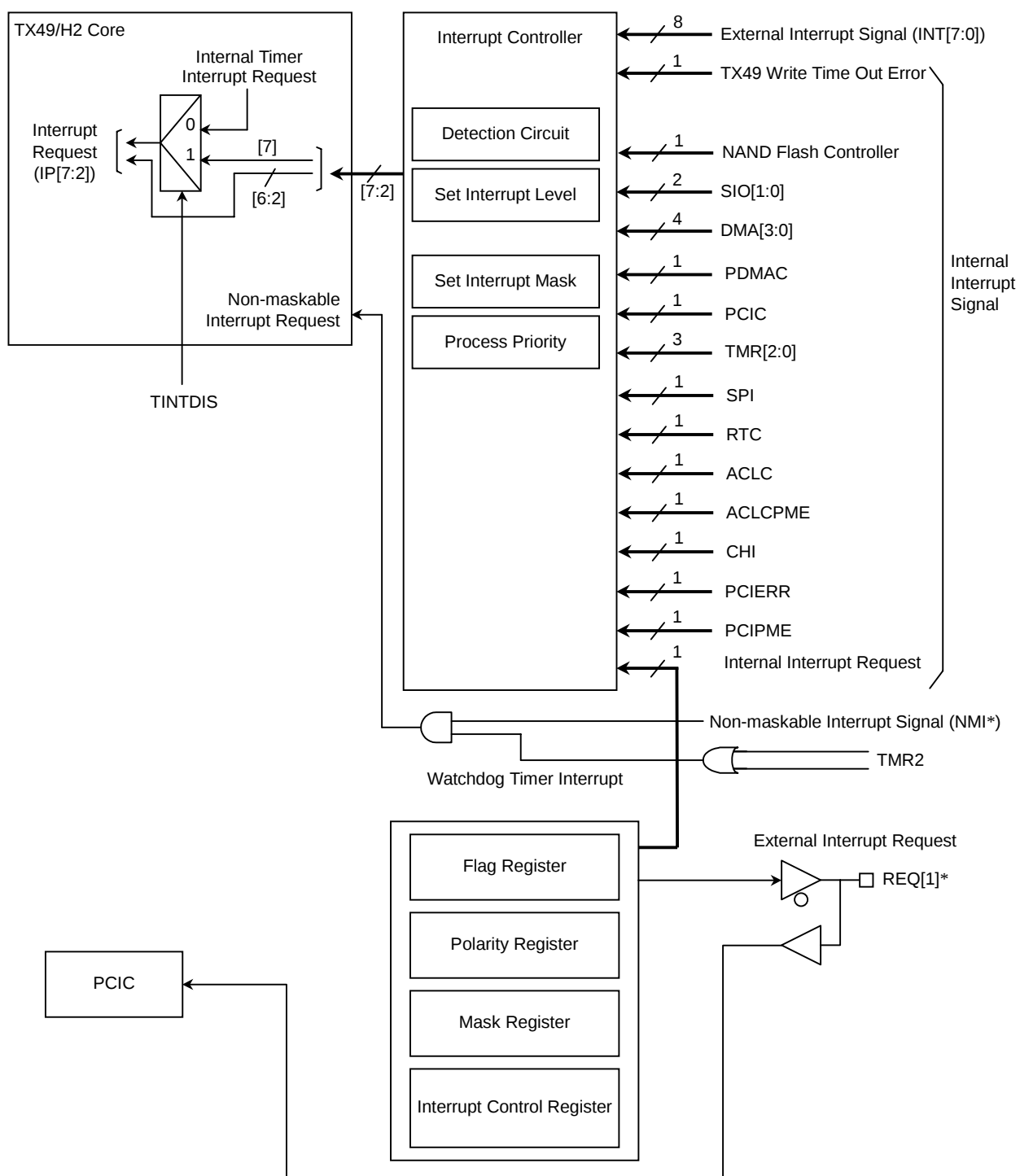
Figure 15.2.1 Interrupt Controller Outline
