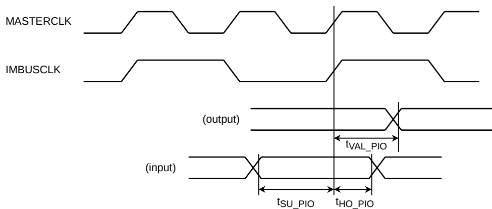
Figure 22.5.12 Timing Diagrams: PIO Interface
