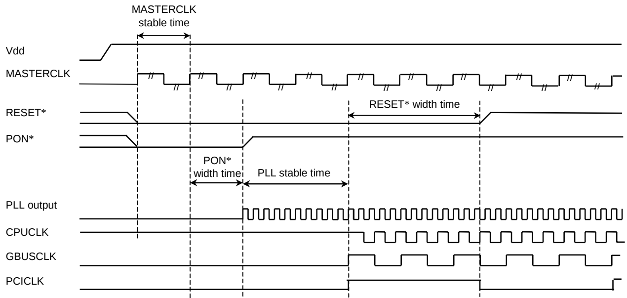
Figure 6.3.1 Power-On Sequence
