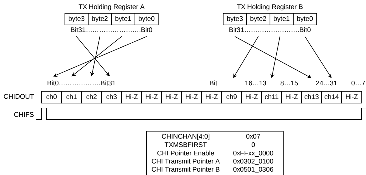
Figure 16.3.1 Transmit TDM Switch Example
