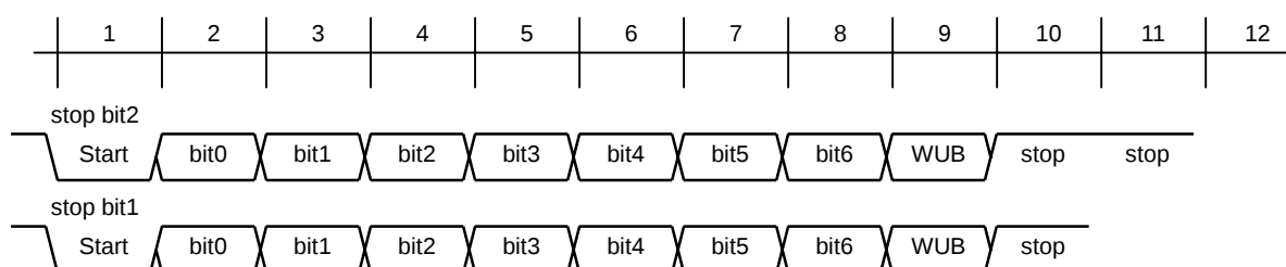
Figure 11.3.1 Data Frame Configuration
