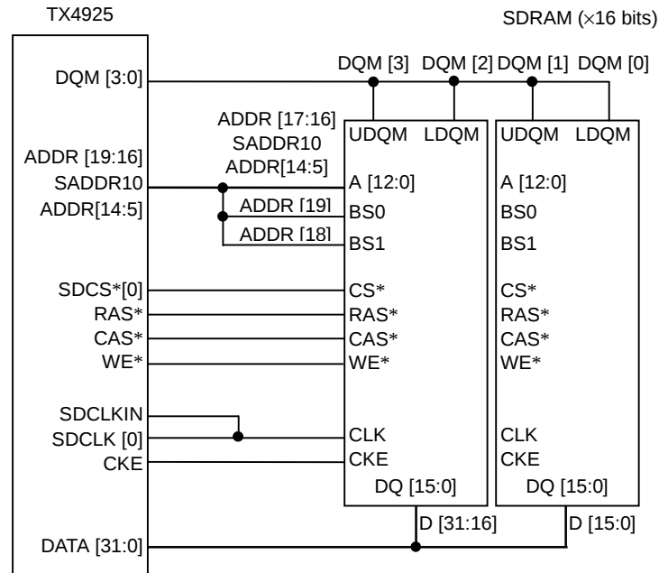
Figure 9.6.1 SDRAM (x16 bits) Connection Example
