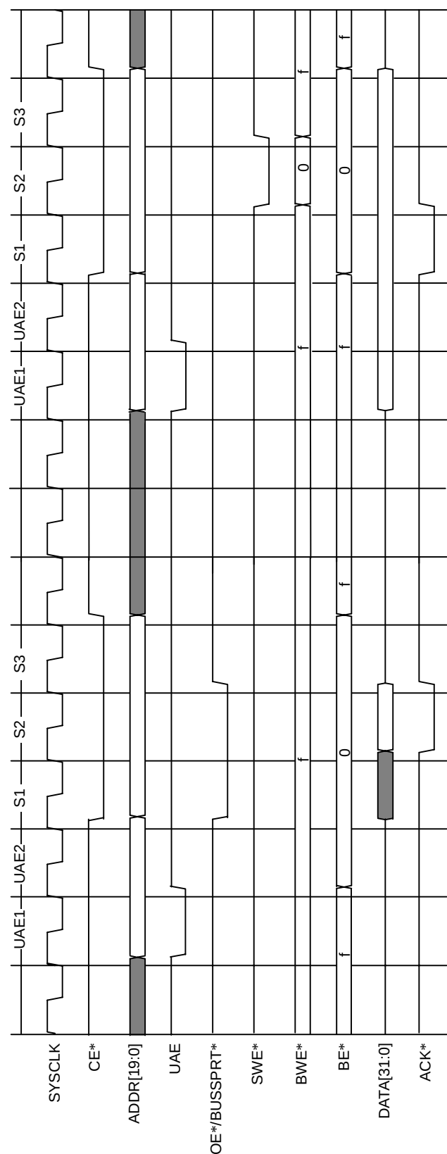
Figure 7.5.1 UAE Signal (CCFG.ACEHOLD=1, PWT: WT=0, SHWT=0, Normal)
