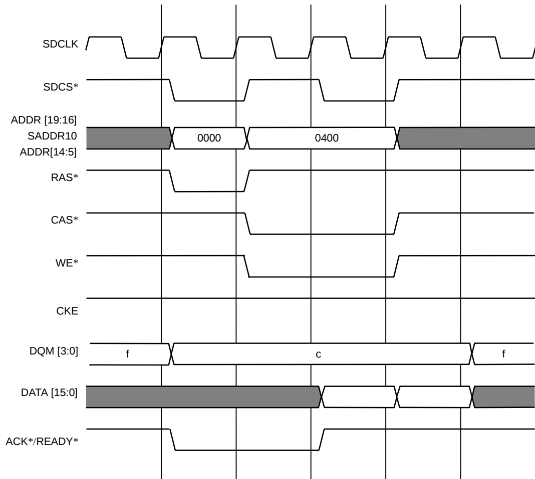
Figure 9.5.10 One-Word Single Write ( t_{\text{RCD}} = 2 , t_{\text{DA}} = 0 , 16-bit Bus)
