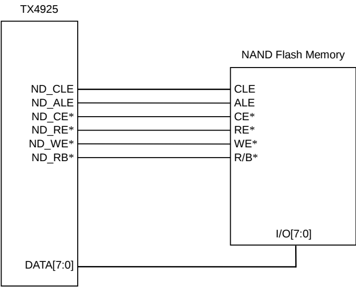
Figure 18.6.1 Example of Using NAND Flash Memory
