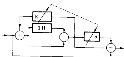
Fig.1 Basic Block Diagram
