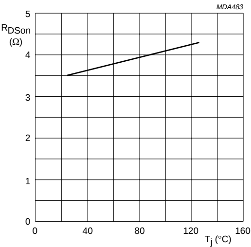
Fig.6 Drain-source on-state resistance as a function of junction temperature, typical values.
