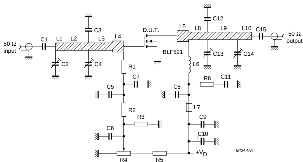
Fig.11 Test circuit for class-B operation.
