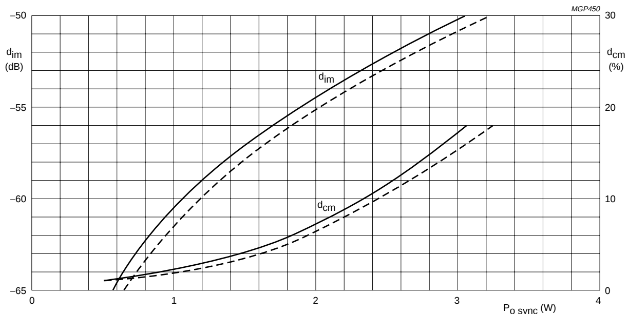
Fig.11 Intermodulation distortion ( d_{\text{im}}^{(1.)} ) and cross-modulation distortion ( d_{\text{cm}}^{(2.)} ) as a function of output power. Typical values; V_{\text{CE}} = 25 \text{ V} ; I_{\text{C}} = 300 \text{ mA} ; f_{\text{vision}} = 860 \text{ MHz} ; --- T_{\text{h}} = 25 \text{ }^{\circ}\text{C} ; — T_{\text{h}} = 70 \text{ }^{\circ}\text{C} .
