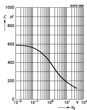
Capacitance
