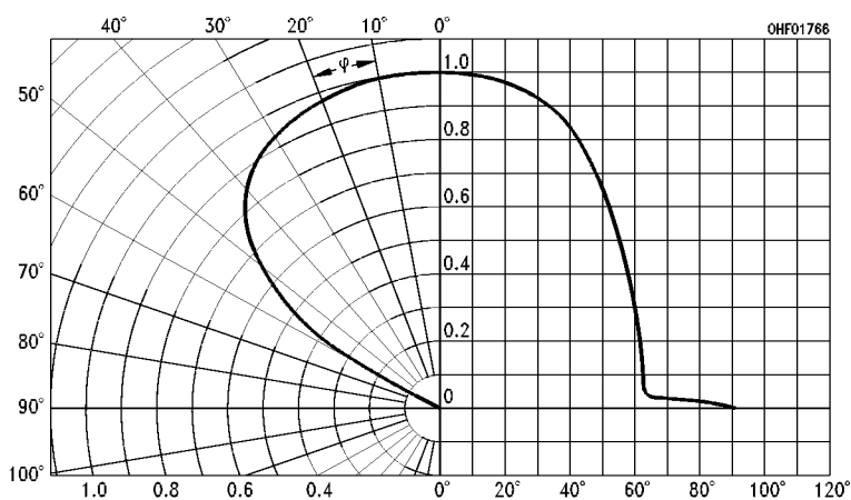
Directional characteristics S_{\text{rel}} = f(\varphi)
