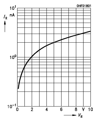
Dark current
