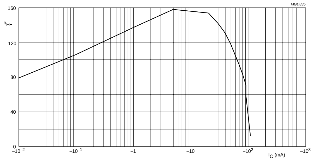
Fig.2 DC current gain; typical value.
