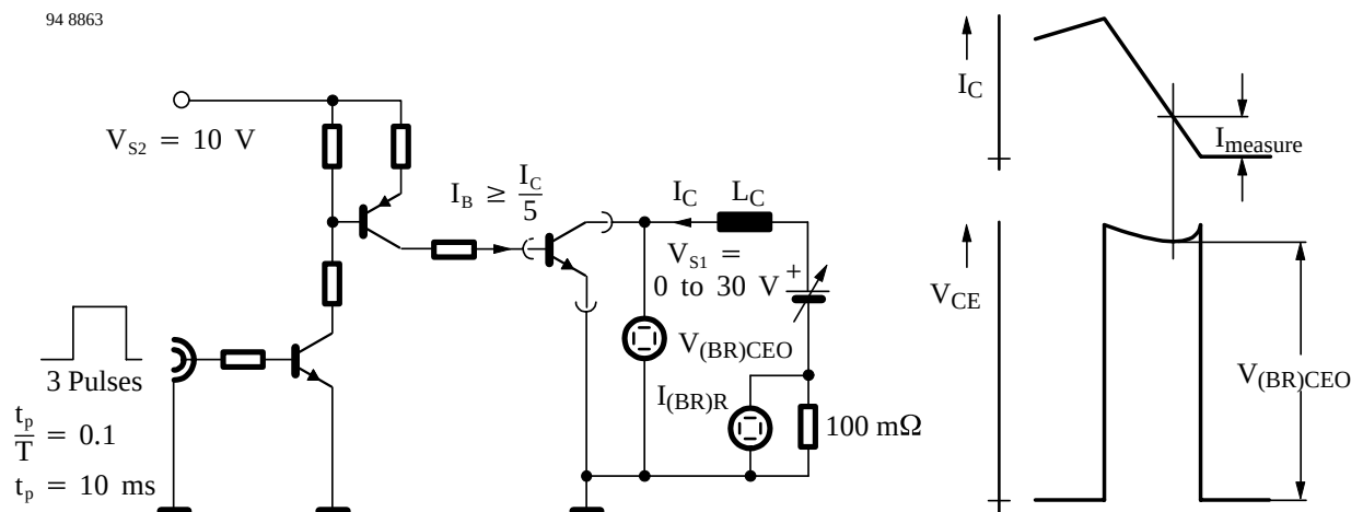
Figure 1. Test circuit for V_{(\text{BR})\text{CE0}}
