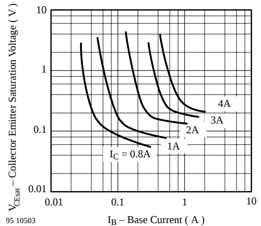
Figure 8. V_{\text{CEsat}} vs. I_{\text{B}}
