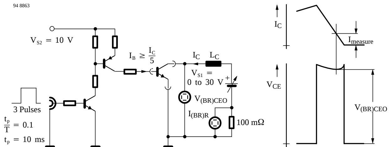
Figure 1. Test circuit for V_{\text{(BR)CE0}}
