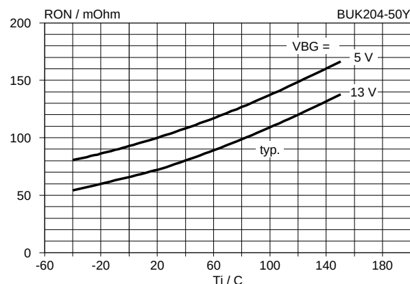
Fig.9. Typical on-state resistance, t_p = 300 \mu s . R_{ON} = f(T) ; parameter V_{BG} ; condition I_L = 1 A
