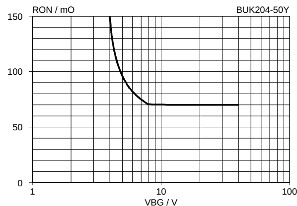
Fig.8. Typical on-state resistance, T_j = 25^\circ\text{C} . R_{ON} = f(V_{BG}) ; conditions: I_l = 5\text{ A} ; t_n = 300\text{ }\mu\text{s}
