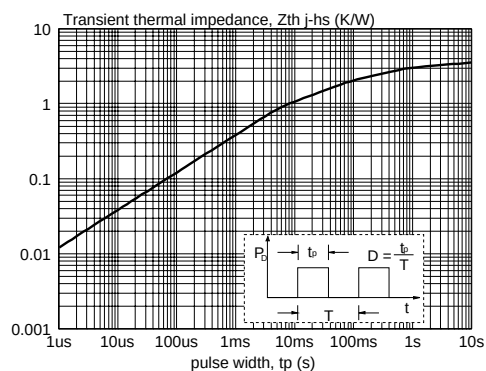
Fig.10. Modulator transient thermal impedance Z_{th} = f(t_p)
