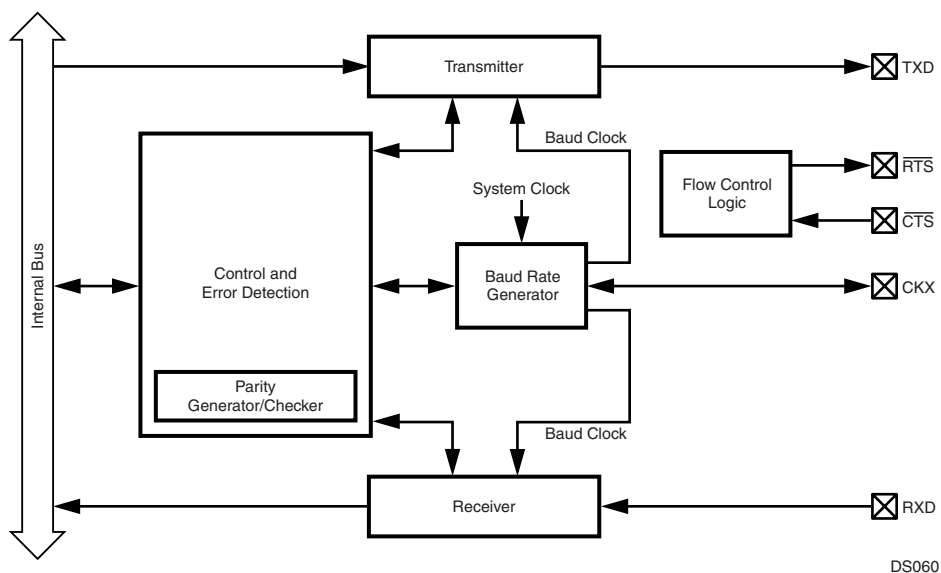
Figure 71. UART Block Diagram
