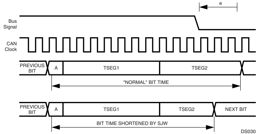
Figure 41. Resynchronization ( e < -SJW )
