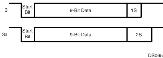
Figure 76. 9-bit Data Frame Options
