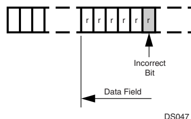
Figure 58. EBID Example
