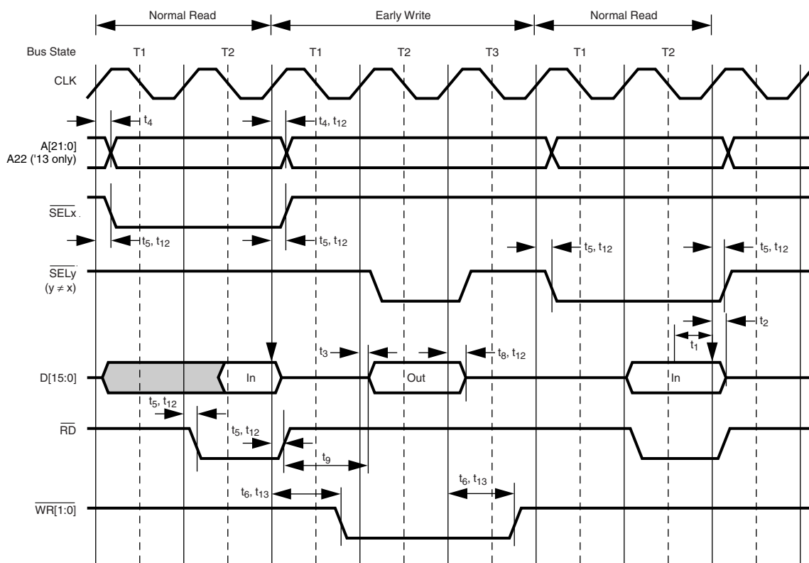
Figure 126. Early Write Between Normal Read Cycles (No Wait States)
