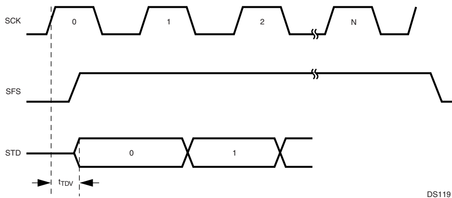
Figure 114. Transmit Timing, Long Frame Sync
