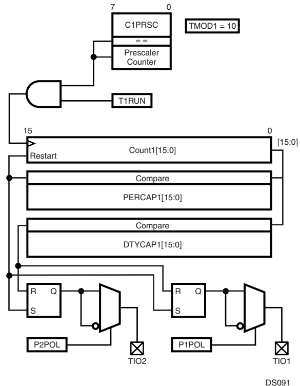
Figure 102. VTU 16-bit PWM Mode
