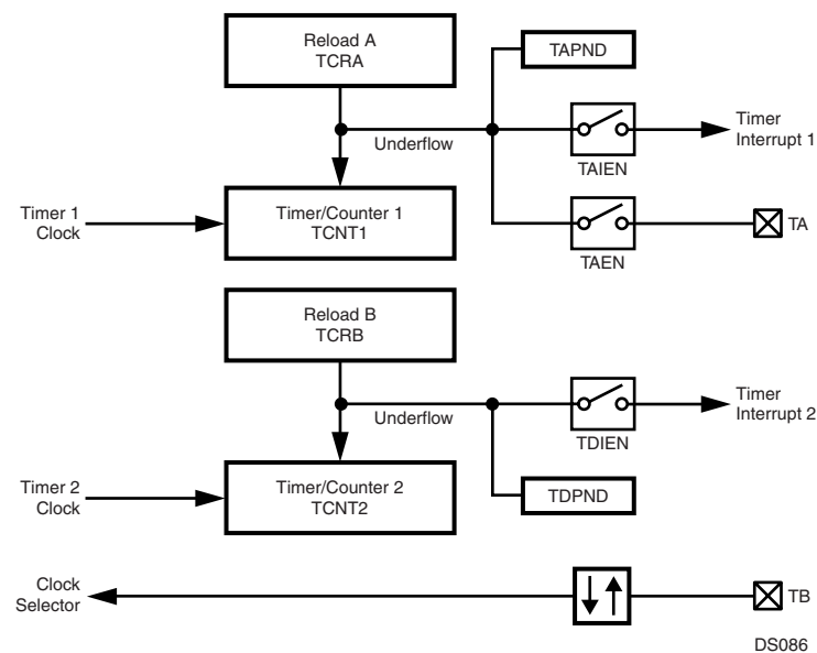
Figure 97. Dual-Independent Timer/Counter Mode
