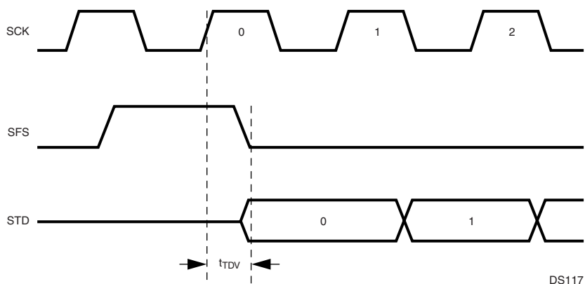
Figure 112. Transmit Timing, Short Frame Sync
