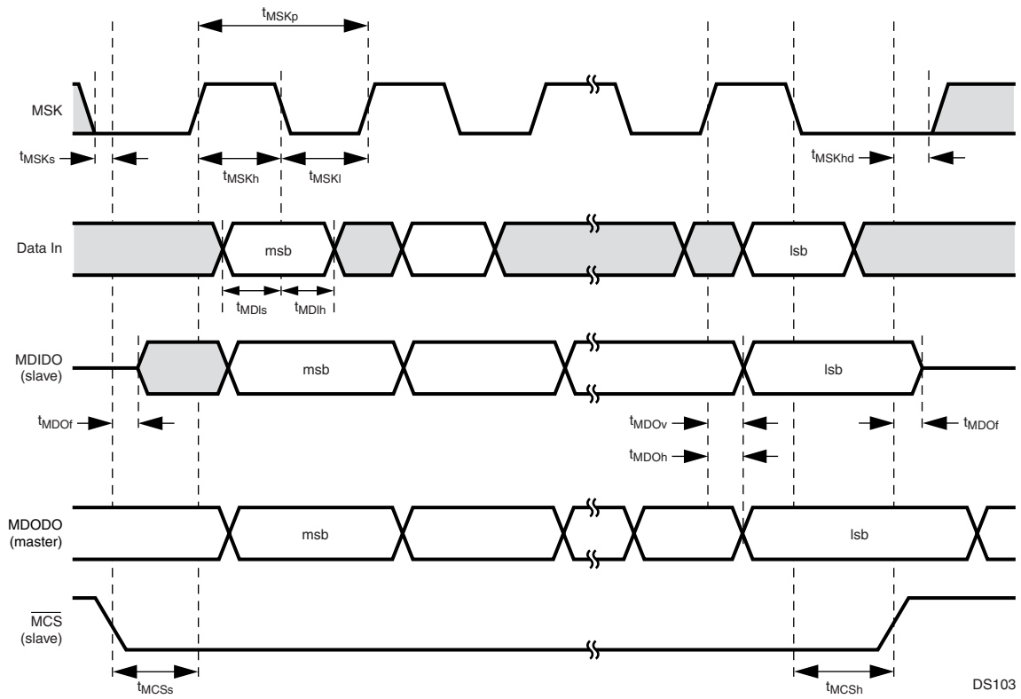
Figure 117. Microwire Transaction Timing, Alternate Mode, SCIDL = 0
