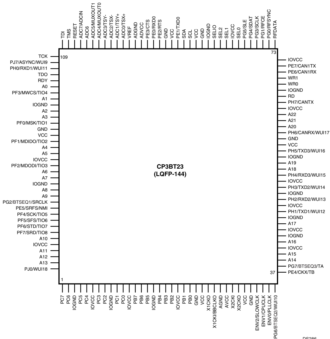
Figure 132. CP3BT23 in the LQFP-144 Package (Top View)
