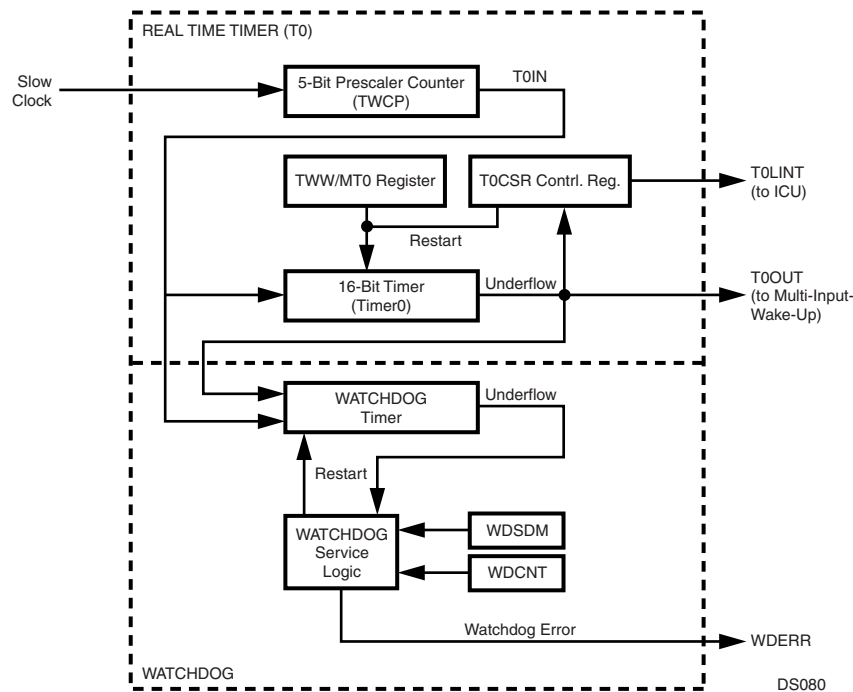
Figure 91. Timing and Watchdog Module Block Diagram
