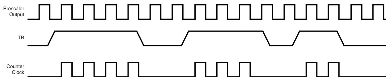
Figure 94. Pulse-Accumulate Mode
