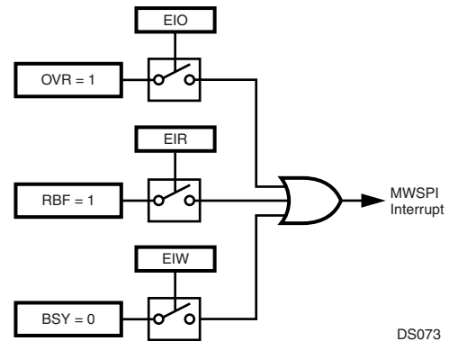
Figure 84. MWSPi Interrupts
