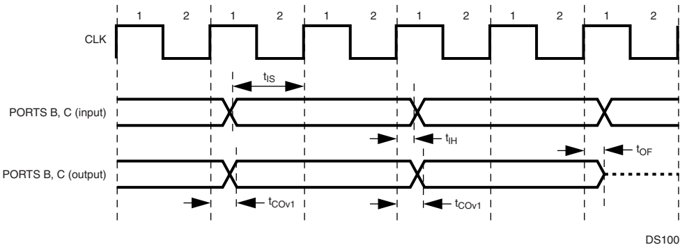
Figure 110. I/O Port Timing
