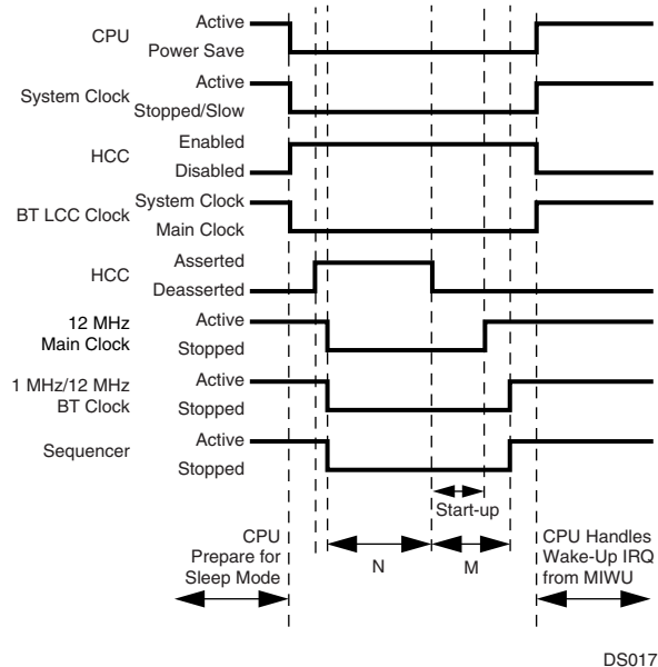
Figure 23. Bluetooth Sleep Mode Sequence
