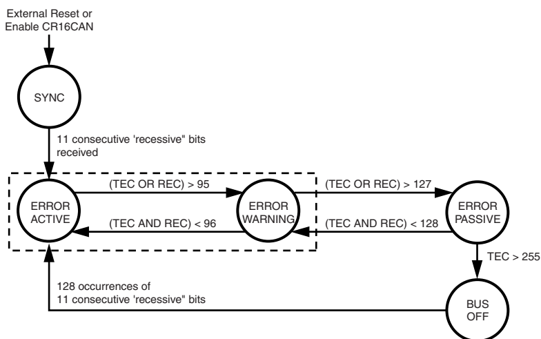
Figure 38. Bus States
