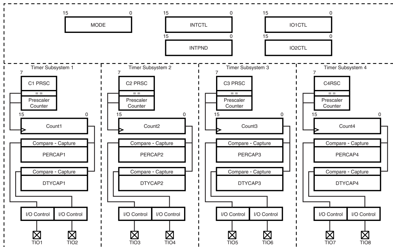
Figure 99. Versatile Timer Unit Block Diagram
