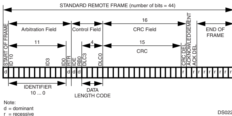
Figure 33. Standard Remote Frame
