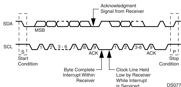
Figure 88. ACCESS.bus Data Transaction
