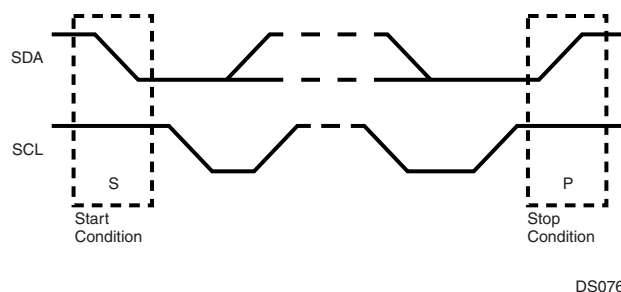
Figure 87. Start and Stop Conditions
