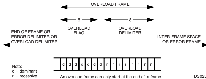
Figure 36. Overload Frame
