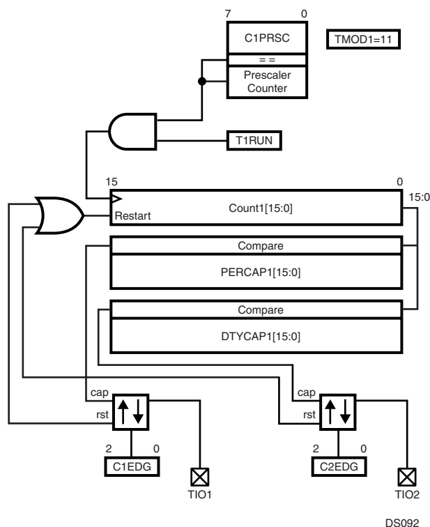
Figure 103. VTU Dual 16-bit Capture Mode
