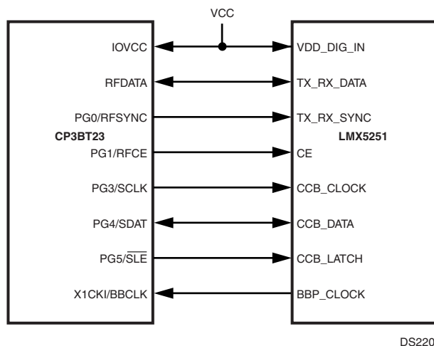
Figure 11. LMX5251 Interface
