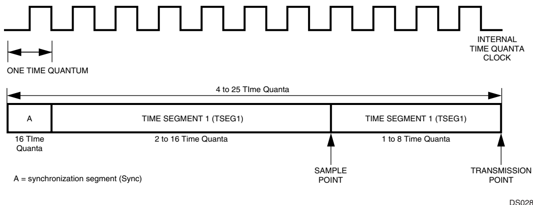
Figure 39. Bit Timing
