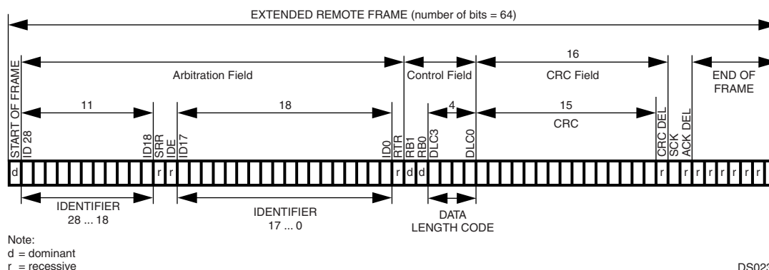
Figure 34. Extended Remote Frame
