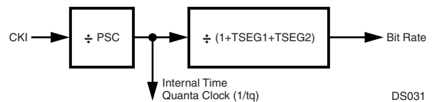
Figure 42. CAN Prescaler
