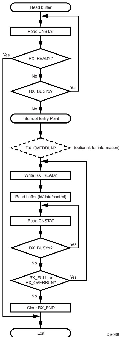
Figure 49. Buffer Read Routine (BUFFLOCK Disabled)
