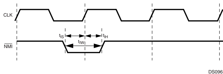
Figure 106. \overline{\text{NMI}} Signal Timing
