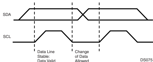
Figure 86. Bit Transfer
