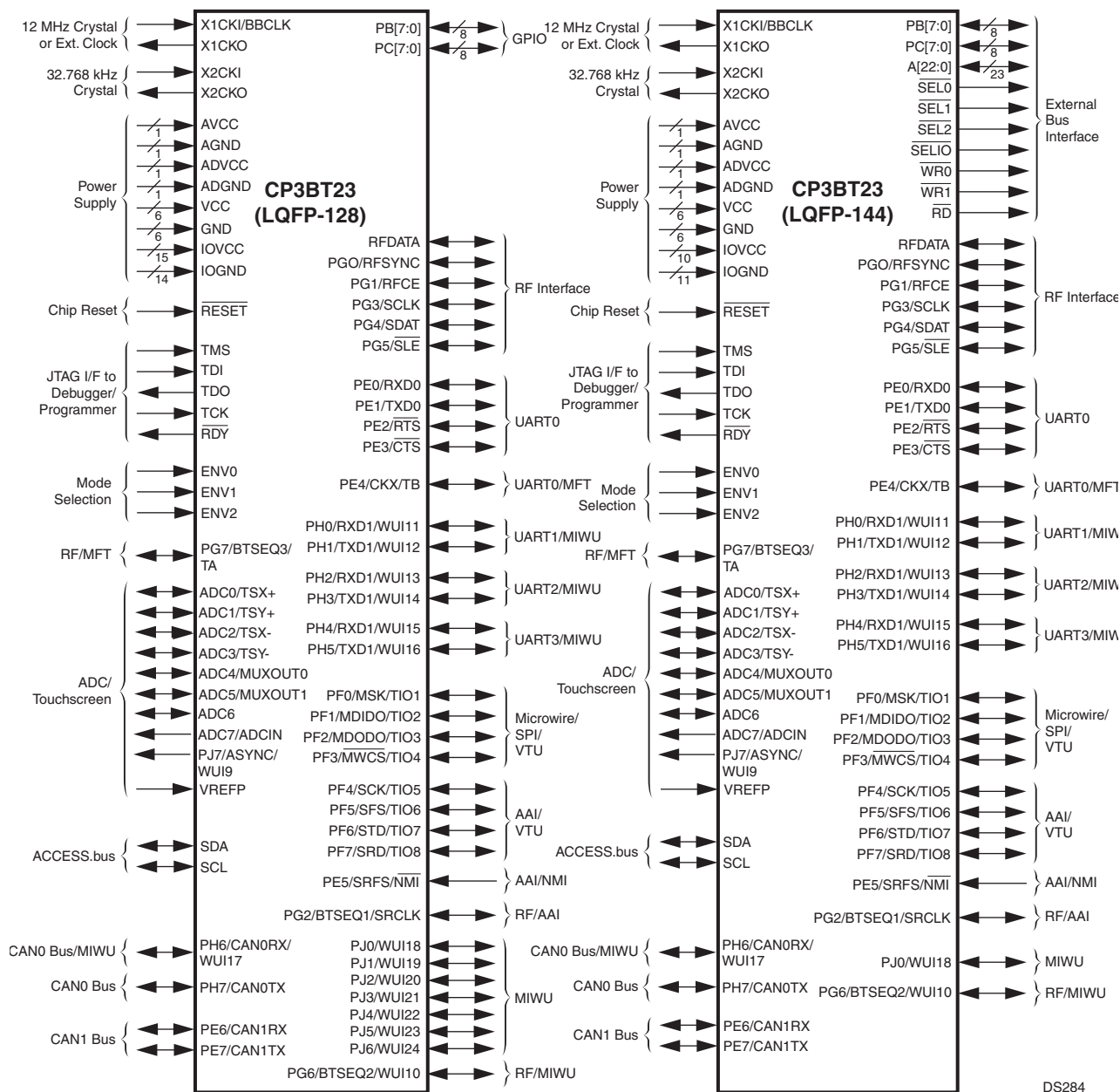
Figure 1. CP3BT23 Device Signals
