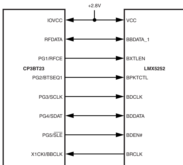
Figure 12. LMX5252 Interface
