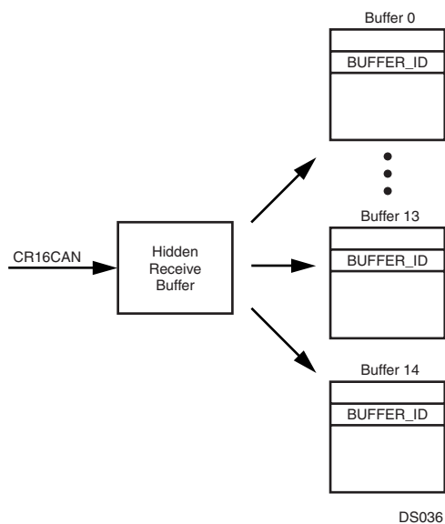
Figure 47. Receive Buffer
