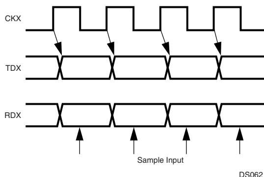
Figure 73. UART Synchronous Communication
