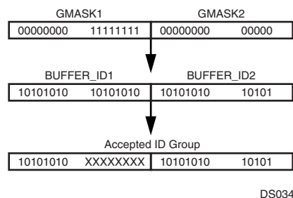
Figure 45. Acceptance of a Group of Identifiers
