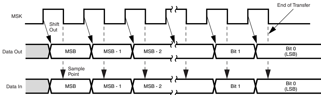
Figure 82. Alternate Mode (SCIDL = 0)
