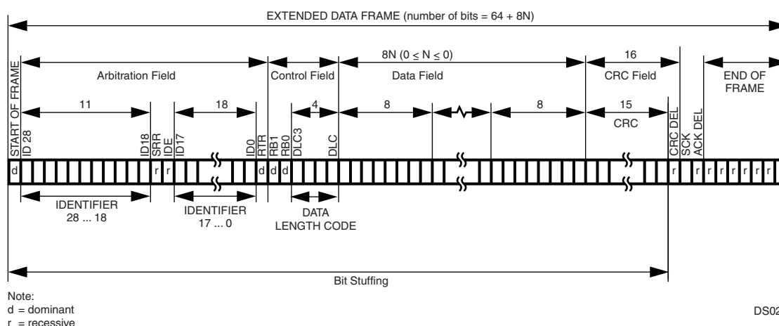
Figure 32. Extended Data Frame
