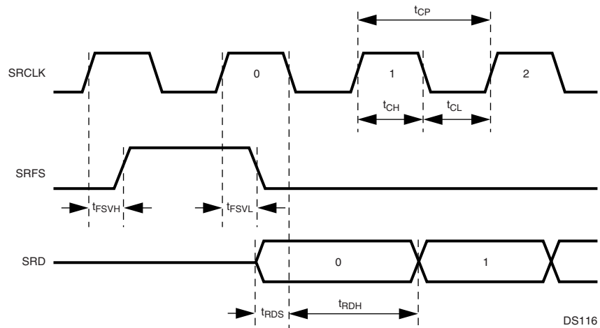
Figure 111. Receive Timing, Short Frame Sync
