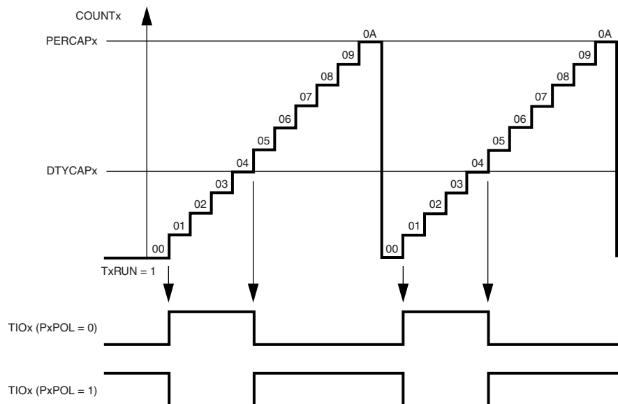
Figure 100. VTU PWM Generation
