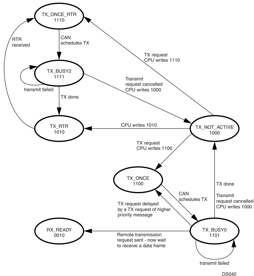
Figure 53. Transmit Buffer States
