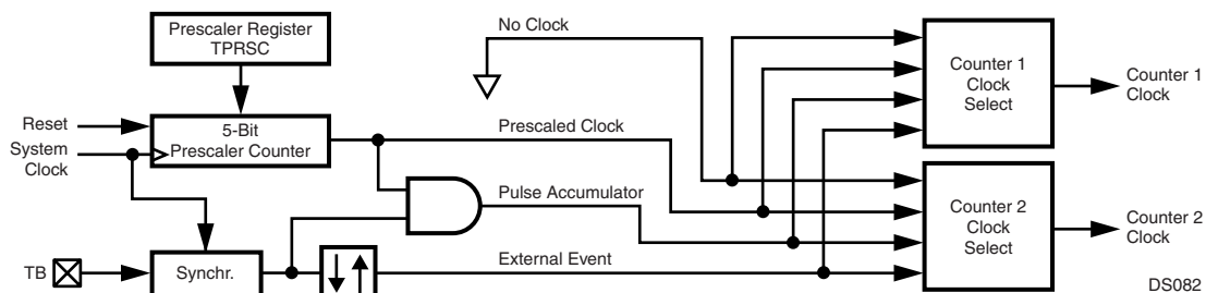
Figure 93. Multi-Function Timer Clock Source
