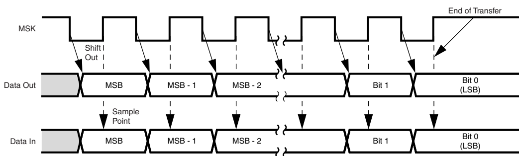
Figure 81. Normal Mode (SCIDL = 1)
