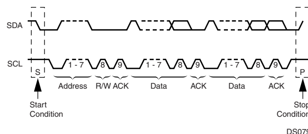
Figure 90. A Complete ACCESS.bus Data Transaction
