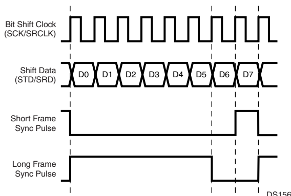
Figure 66. Short and Long Frame Sync Pulses
