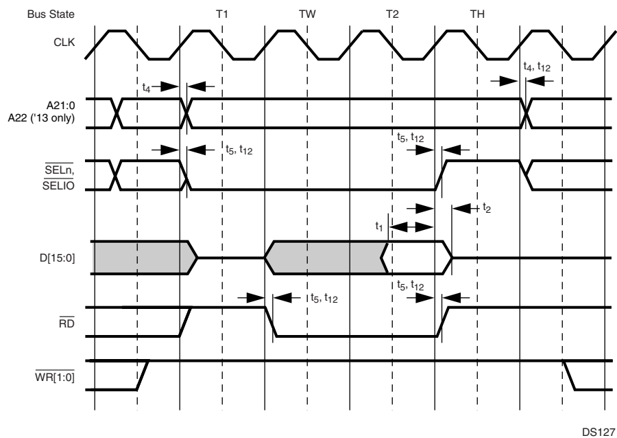
Figure 129. Normal Read Cycle (Wait Cycle Followed by Hold Cycle)
