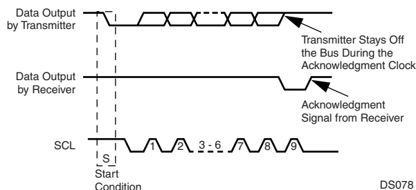
Figure 89. ACCESS.bus Acknowledge Cycle
