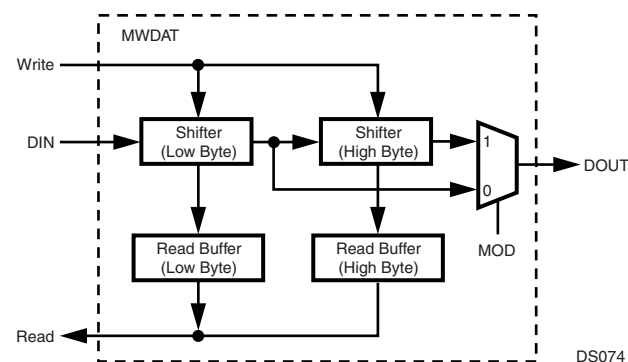
Figure 85. MWDAT Register
