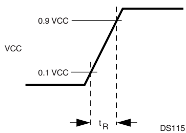
Figure 108. Power-On Reset
