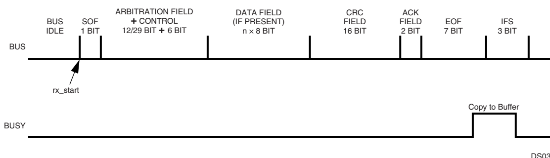
Figure 48. Receive Timing
