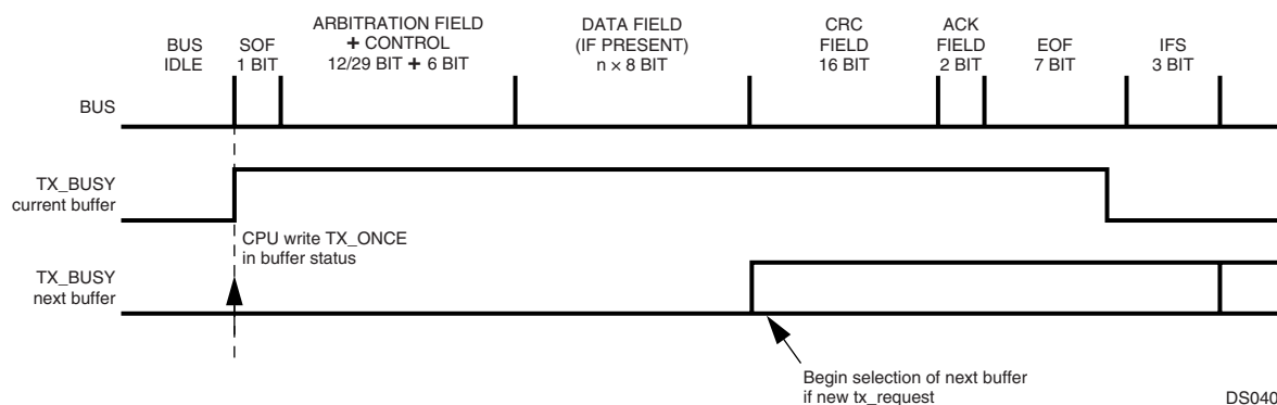
Figure 51. Data Transmission
