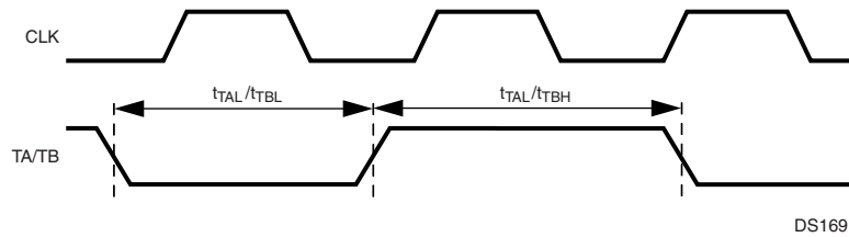
Figure 124. Multi-Function Timer Input Timing
