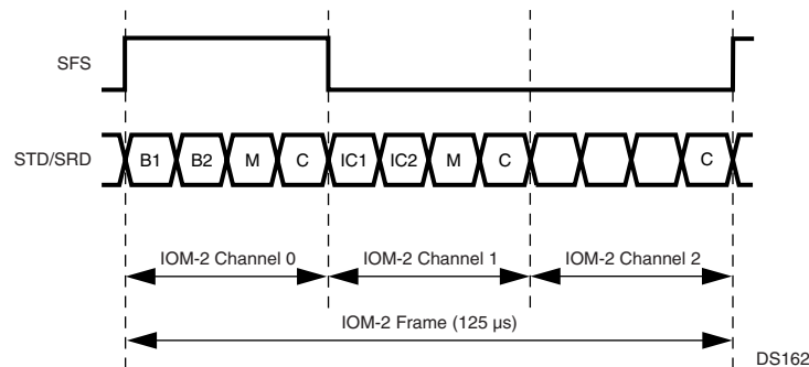
Figure 68. IOM-2 Frame Structure
