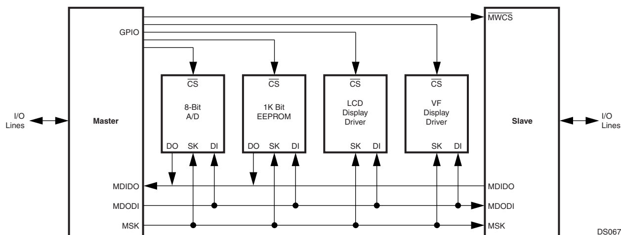
Figure 78. Microwire Interface
