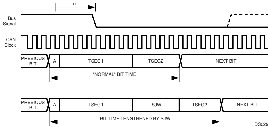
Figure 40. Resynchronization ( e > SJW )
