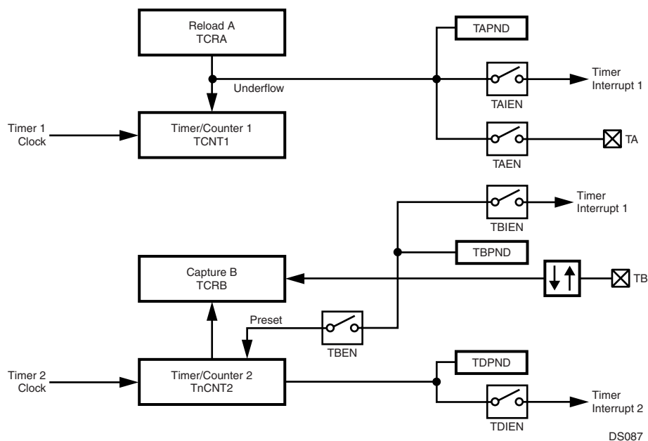
Figure 98. Input Capture Plus Timer Mode
