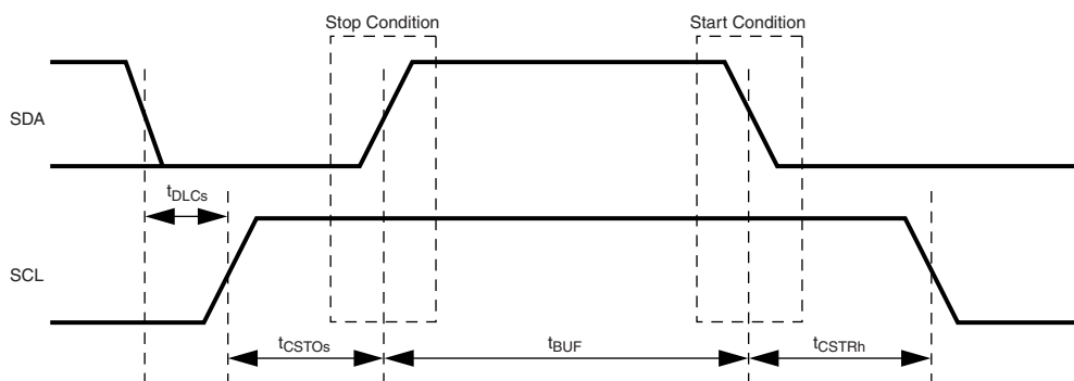
Figure 121. ACB Start and Stop Condition Timing
