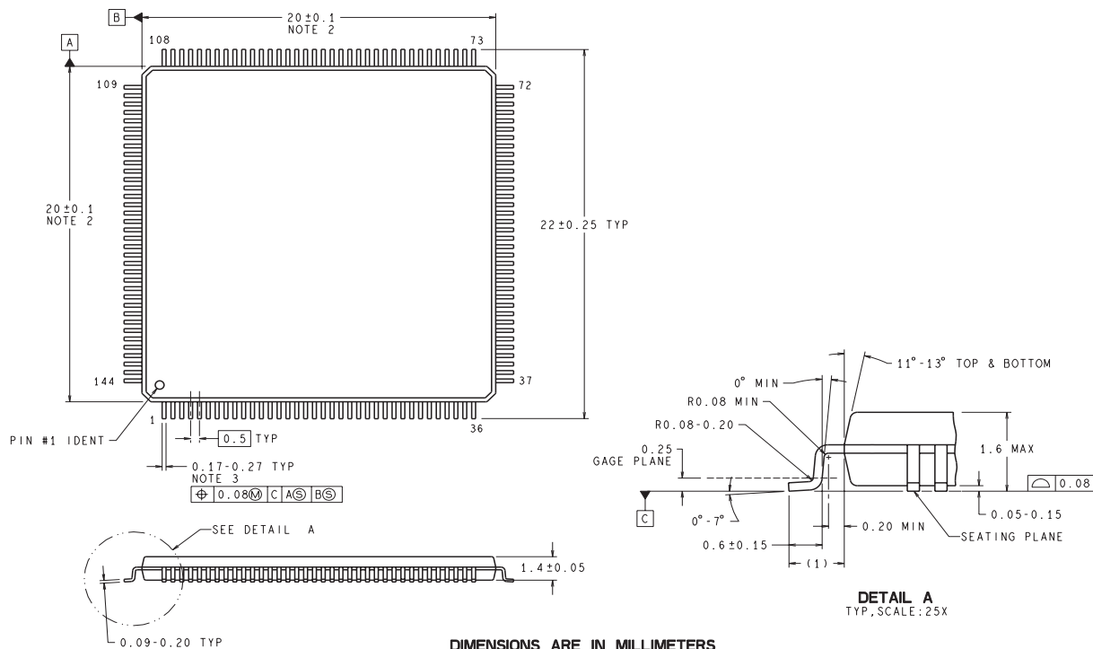
Figure 134. LQFP-144 Package
