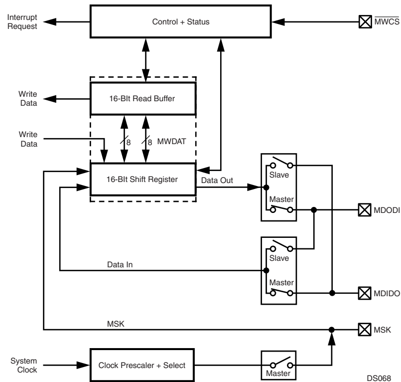
Figure 79. Microwire Block Diagram
