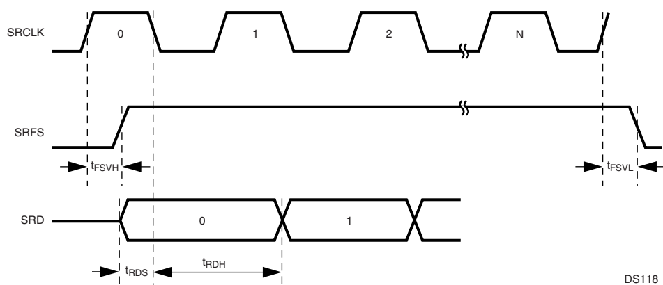
Figure 113. Receive Timing, Long Frame Sync
