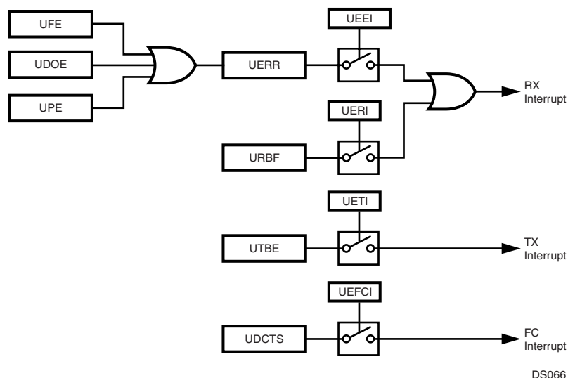
Figure 77. UART Interrupts
