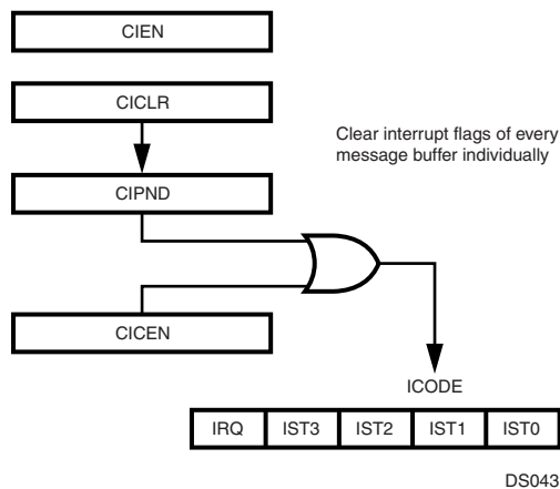
Figure 54. Interrupt Management
