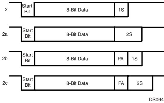
Figure 75. 8-Bit Data Frame Options
