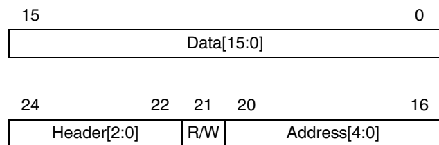
Figure 13. Serial Interface Protocol Format
