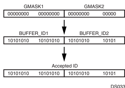
Figure 44. Acceptance of a Single Identifier
