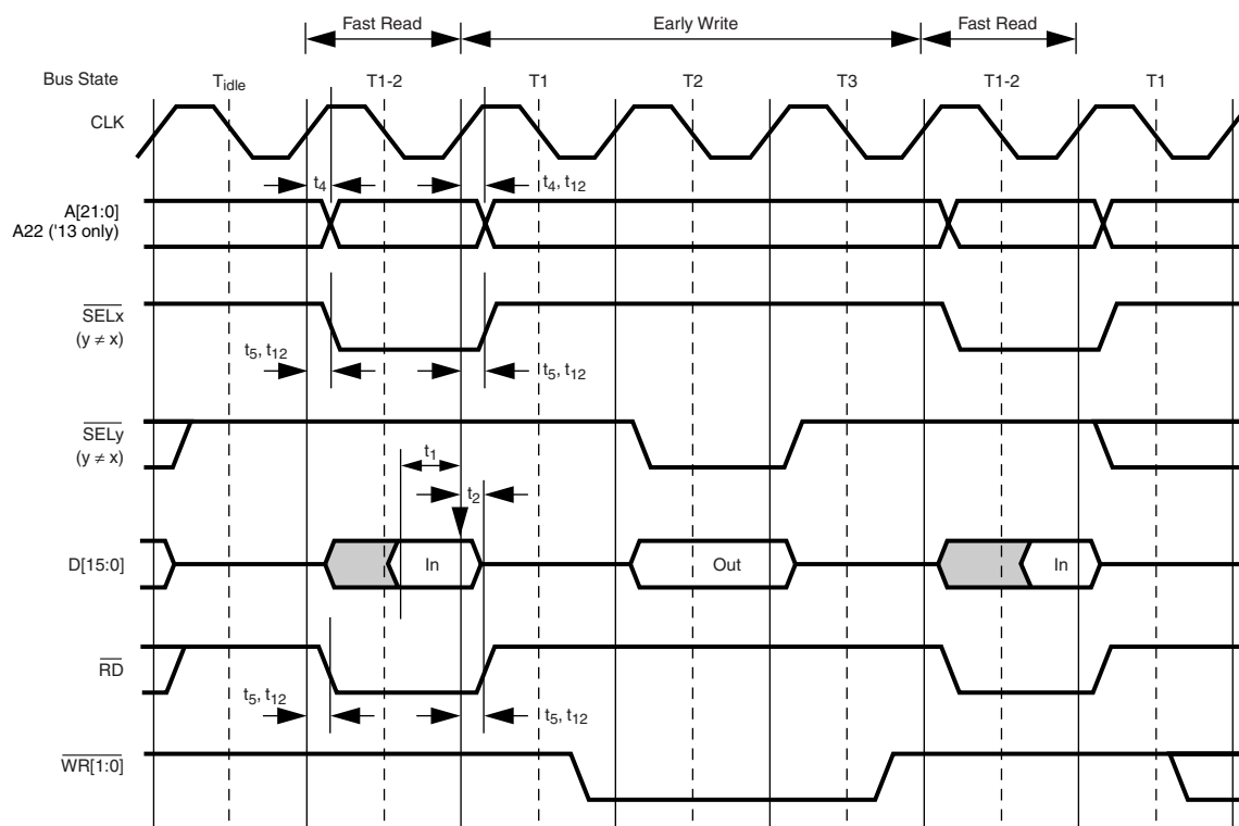
Figure 130. Early Write Between Fast Read Cycles
