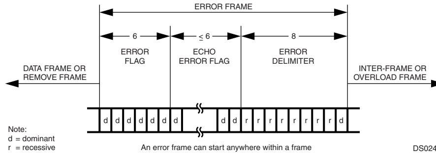
Figure 35. Error Frame
