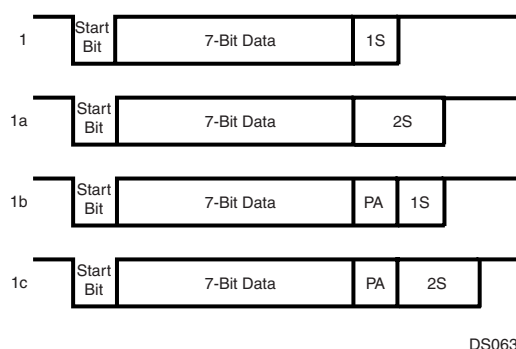
Figure 74. 7-Bit Data Frame Options
