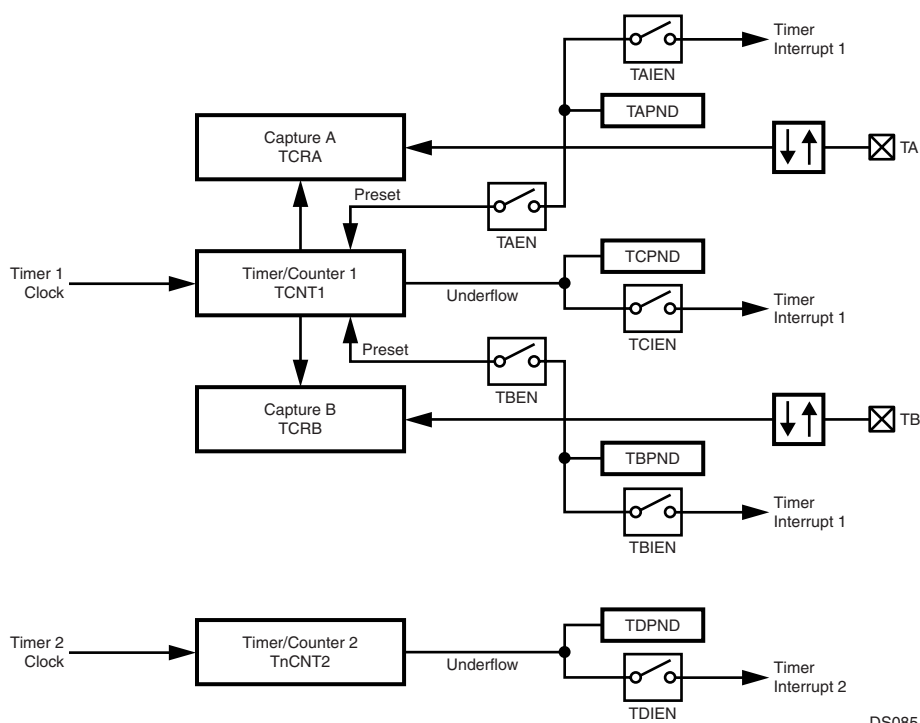
Figure 96. Dual-Input Capture Mode
