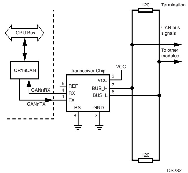
Figure 59. External Transceiver
