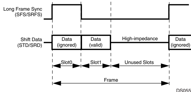
Figure 62. Network Mode Frame
