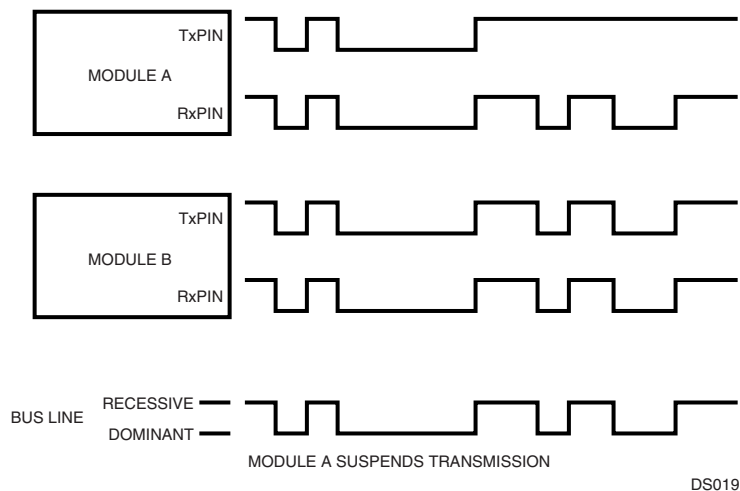
Figure 30. CAN Message Arbitration
