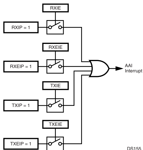
Figure 65. AAI Interrupt Structure
