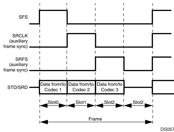
Figure 64. Accessing Three Devices in Network Mode
