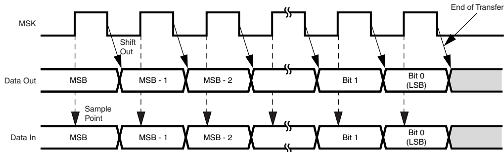
Figure 80. Normal Mode (SCIDL = 0)
