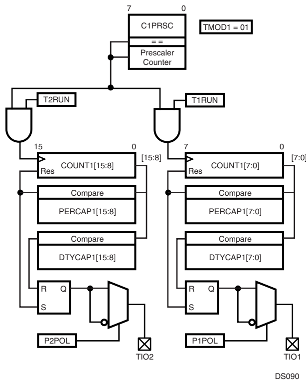
Figure 101. VTU Dual 8-Bit PWM Mode
