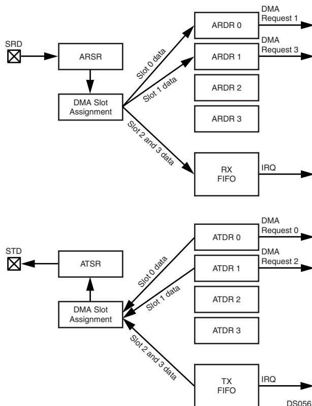
Figure 63. IRQ/DMA Support in Network Mode
