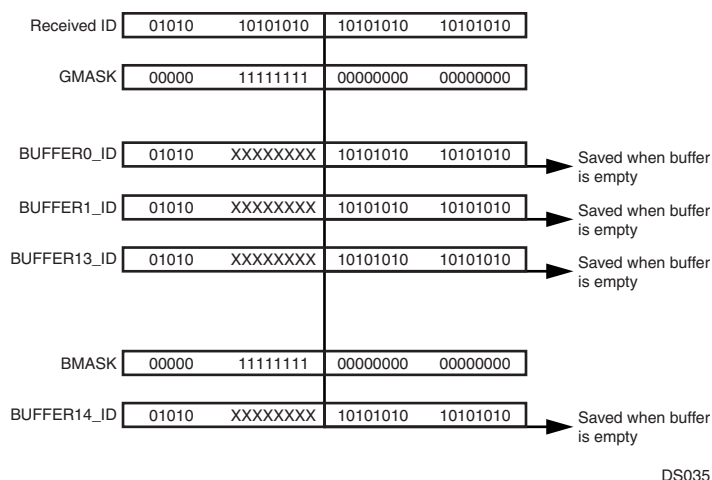
Figure 46. Message Storage with BUFFLOCK Enabled
