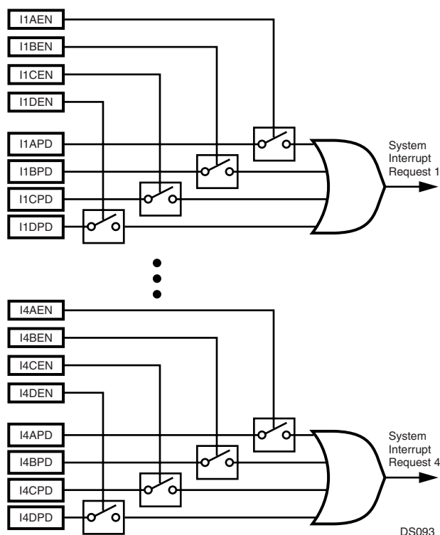
Figure 104. VTU Interrupt Request Structure
