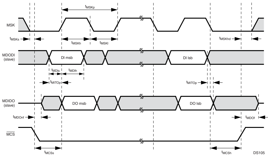
Figure 119. Microwire Transaction Timing, Data Echoed to Output, Normal Mode, SCIDL = 0, ECHO = 1, Slave Mode
