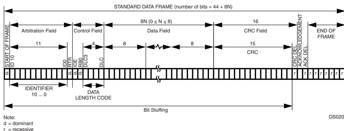
Figure 31. Standard Data Frame
