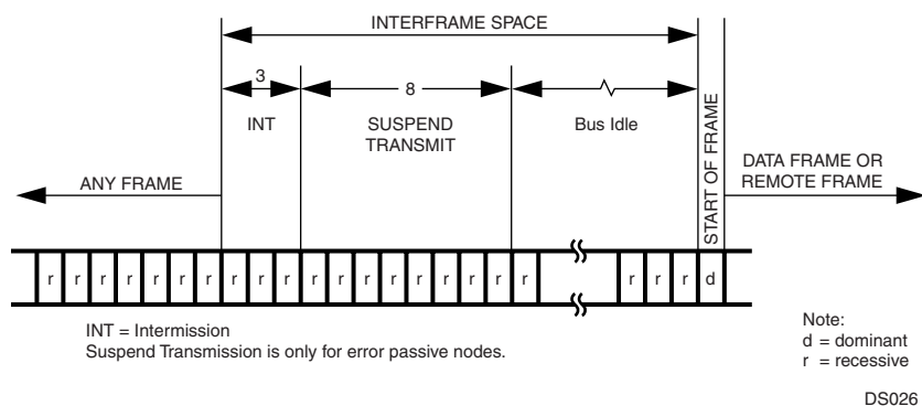
Figure 37. Interframe Space
