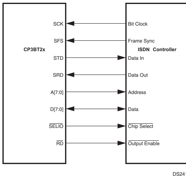
Figure 69. CP3BT23/ISDN Controller Connections
