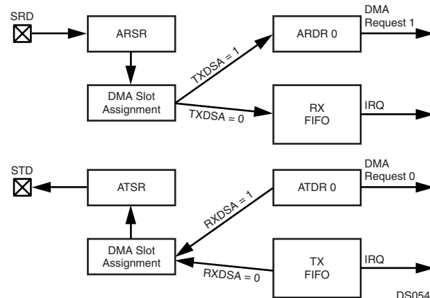
Figure 61. IRQ/DMA Support in Normal Mode
