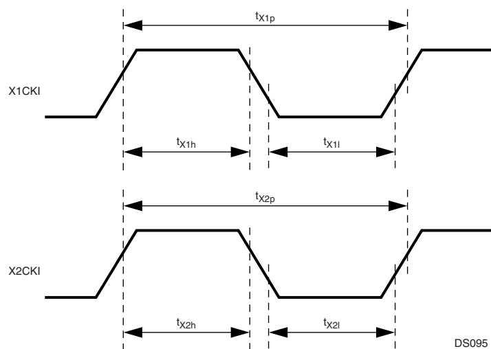
Figure 105. Clock Timing
