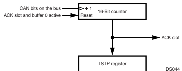
Figure 55. Time Stamp Counter
