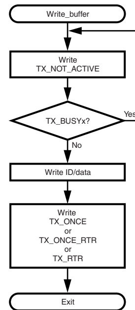
Figure 52. Buffer Write Routine
