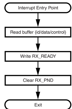
Figure 50. Buffer Read Routine (BUFFLOCK Enabled)
