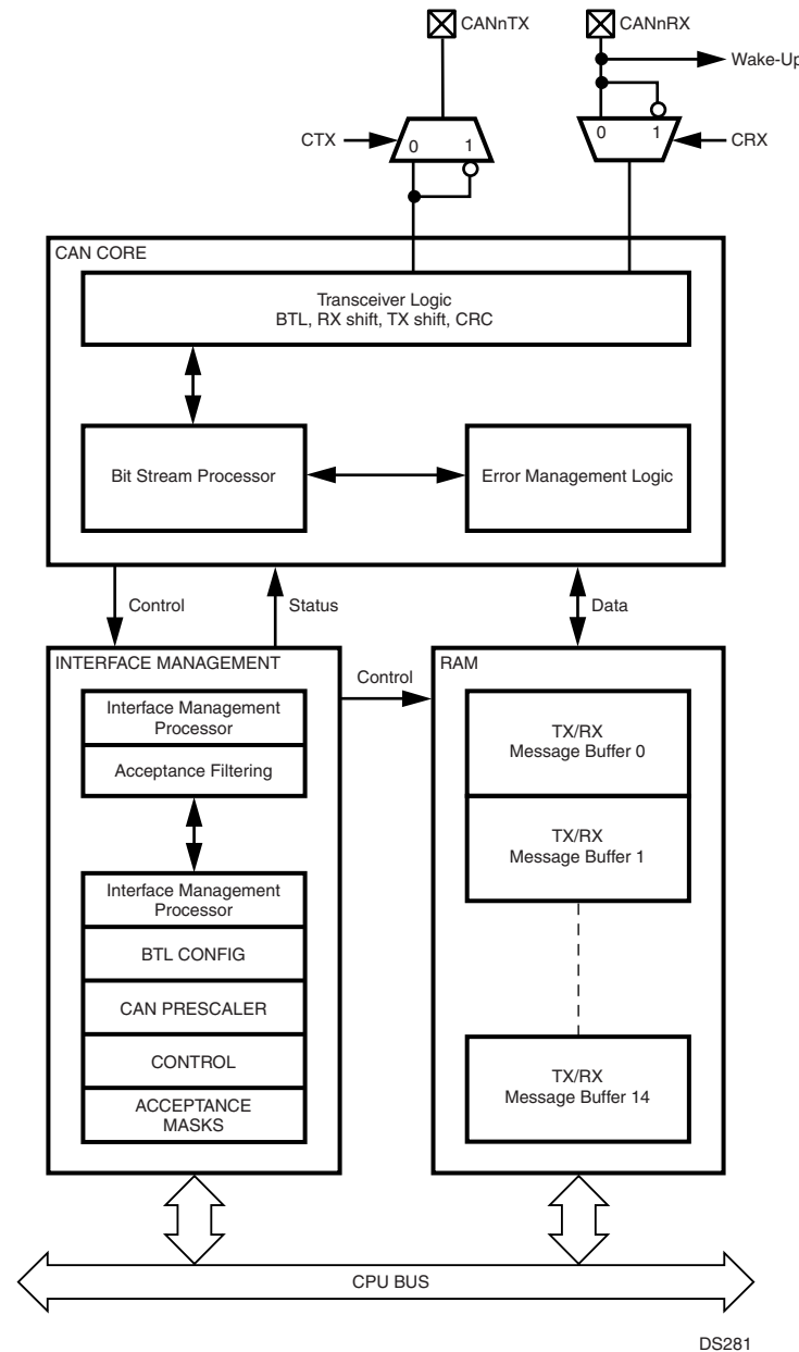
Figure 29. CAN Block Diagram
