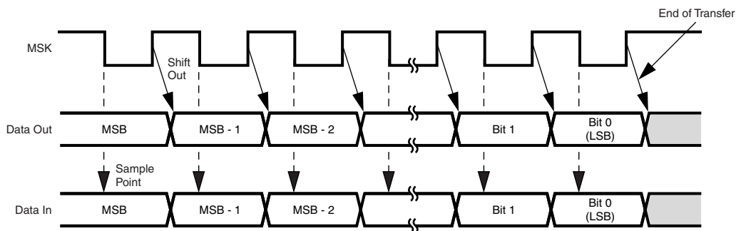
Figure 83. Alternate Mode (SCIDL = 1)
