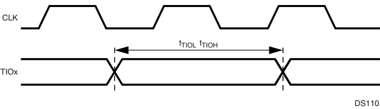
Figure 125. Versatile Timing Unit Input Timing
