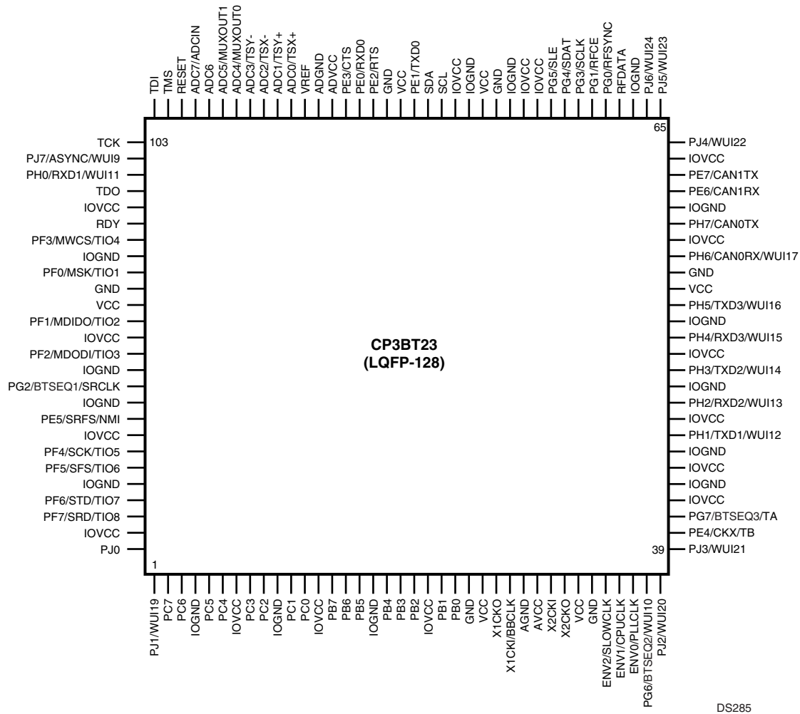
Figure 131. CP3BT23 in the LQFP-128 Package (Top View)
