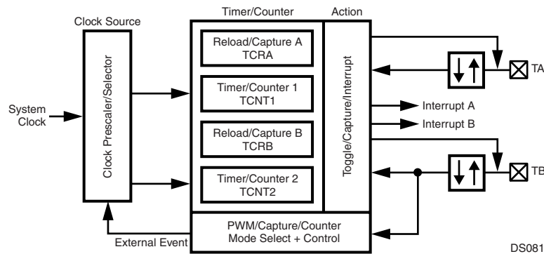
Figure 92. Multi-Function Timer Block Diagram
