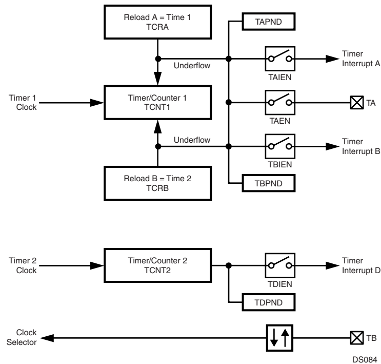
Figure 95. Processor-Independent PWM Mode
