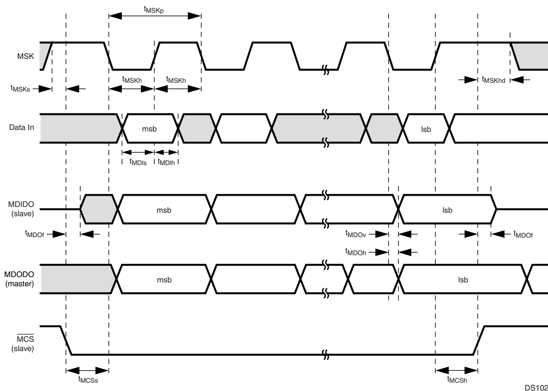
Figure 116. Microwire Transaction Timing, Normal Mode, SCIDL = 1
