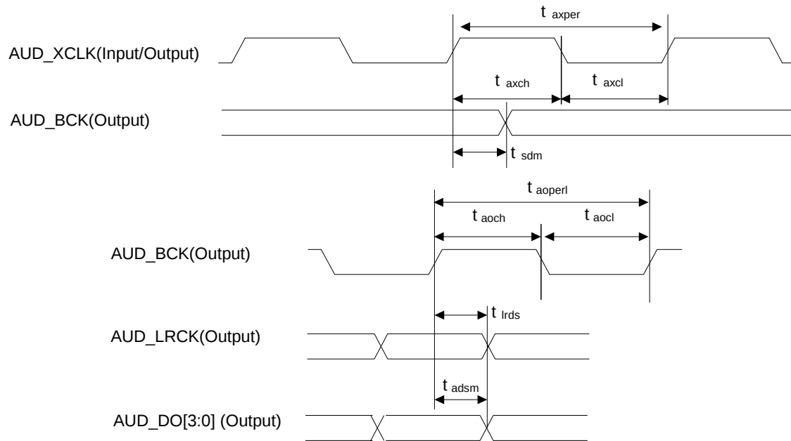
Figure 10. Audio Output Timing
