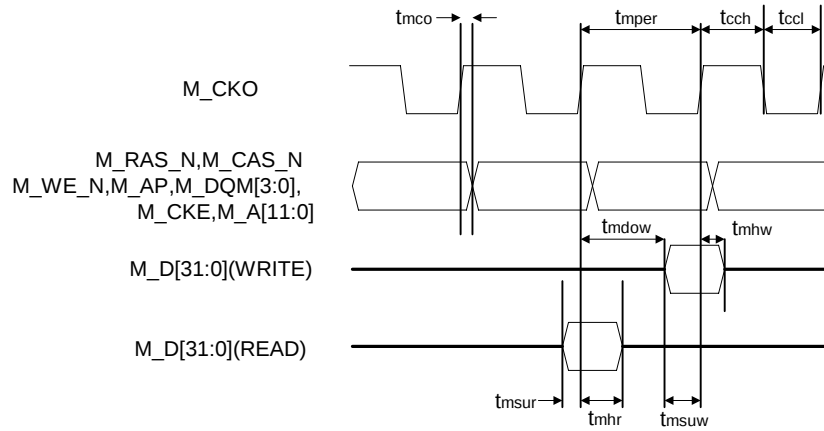
Figure 5. SDRAM Timing
