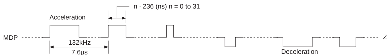
Timing Chart 1-8
