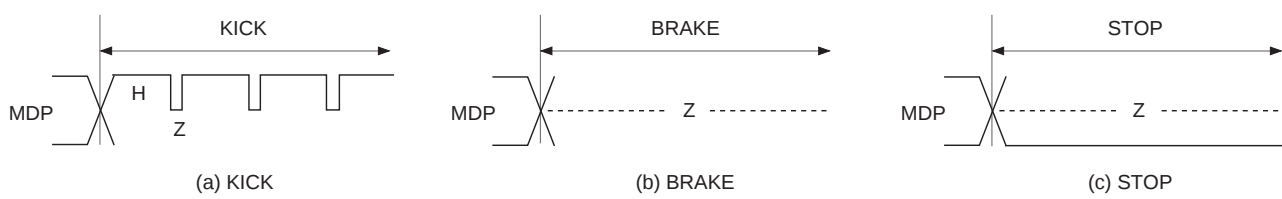
Timing Chart 1-4 CLV-W mode (when following the spindle rotational velocity) LPWR = 1
