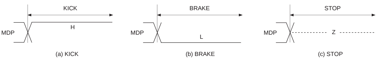
Timing Chart 1-5 CAV-W mode LPWR = 0
