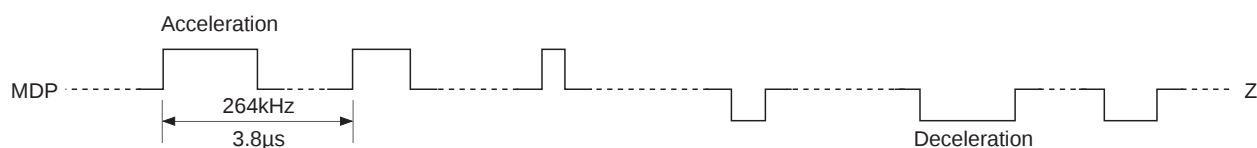
Timing Chart 1-9
