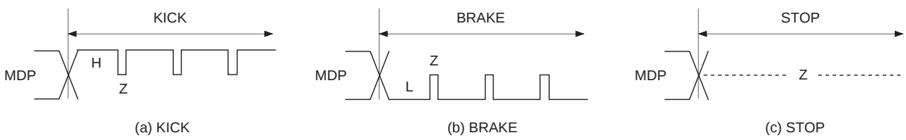
Timing Chart 1-3 CLV-W mode (when following the spindle rotational velocity) LPWR = 0
