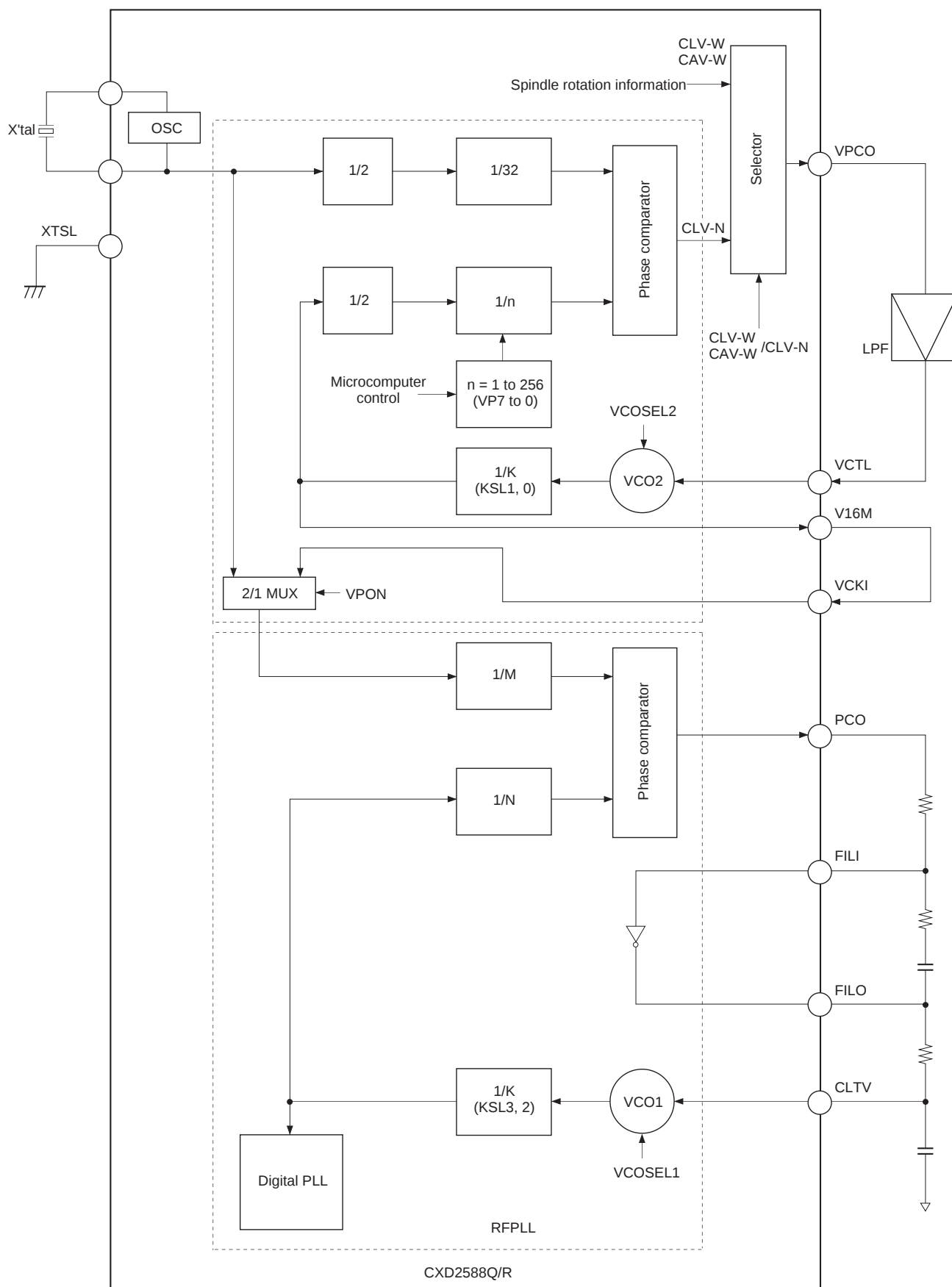
Block Diagram 4-1
