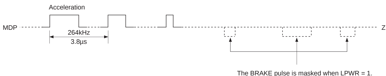
Timing Chart 1-10
