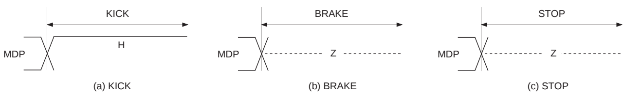
Timing Chart 1-6 CAV-W mode LPWR = 1
