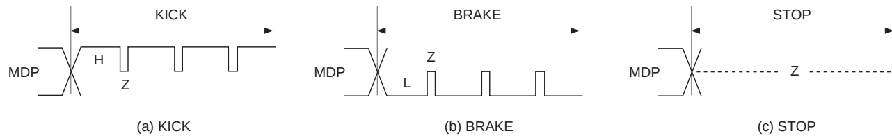
Timing Chart 1-2 CLV-N mode LPWR = 0
