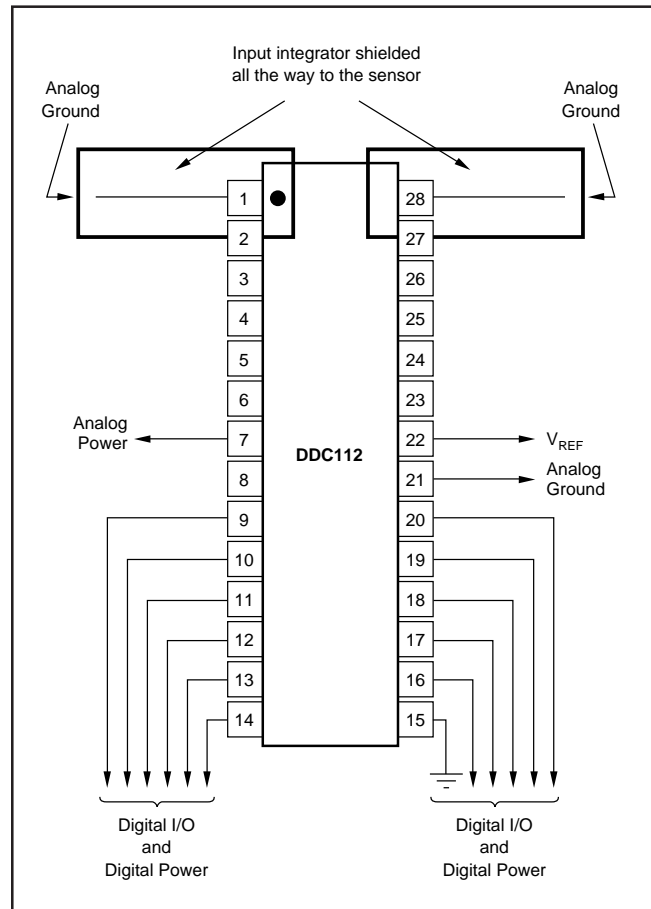
FIGURE 30. Recommended Shield for DDC112 Layout Design.
