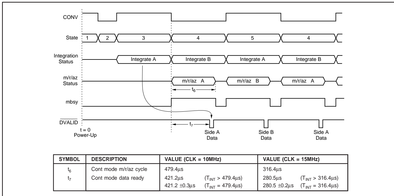
FIGURE 10. Continuous Mode Timing (CONV HIGH at power-up).
