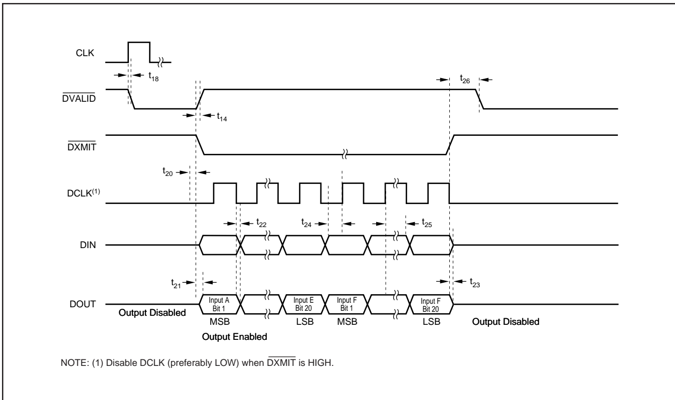
FIGURE 23. Timing Diagram When Using the DIN Function of the DDC112.
