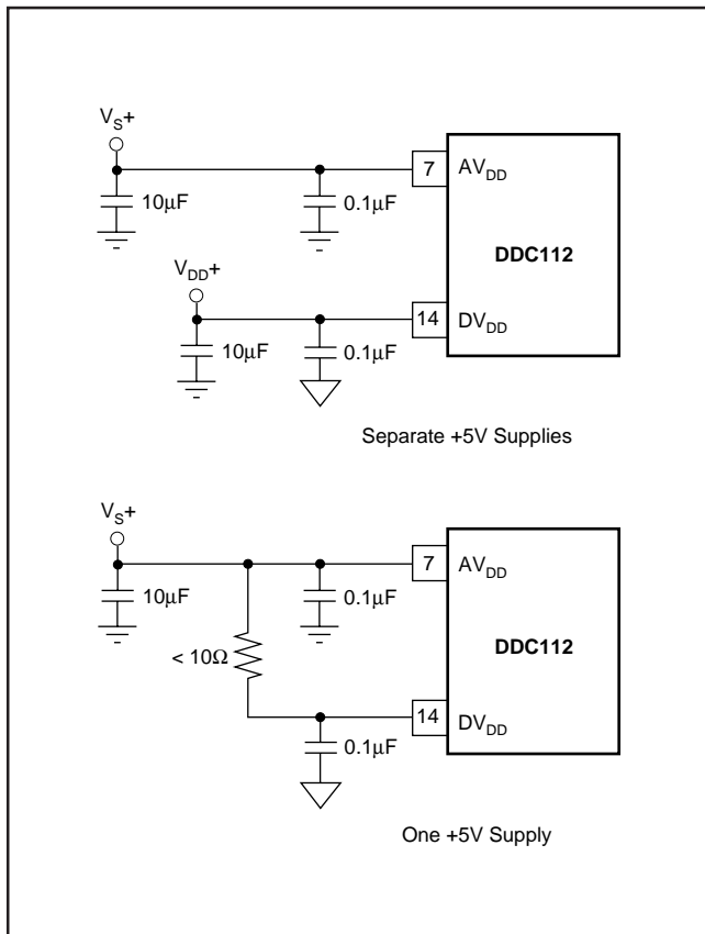
FIGURE 29. Power Supply Connection Options.
