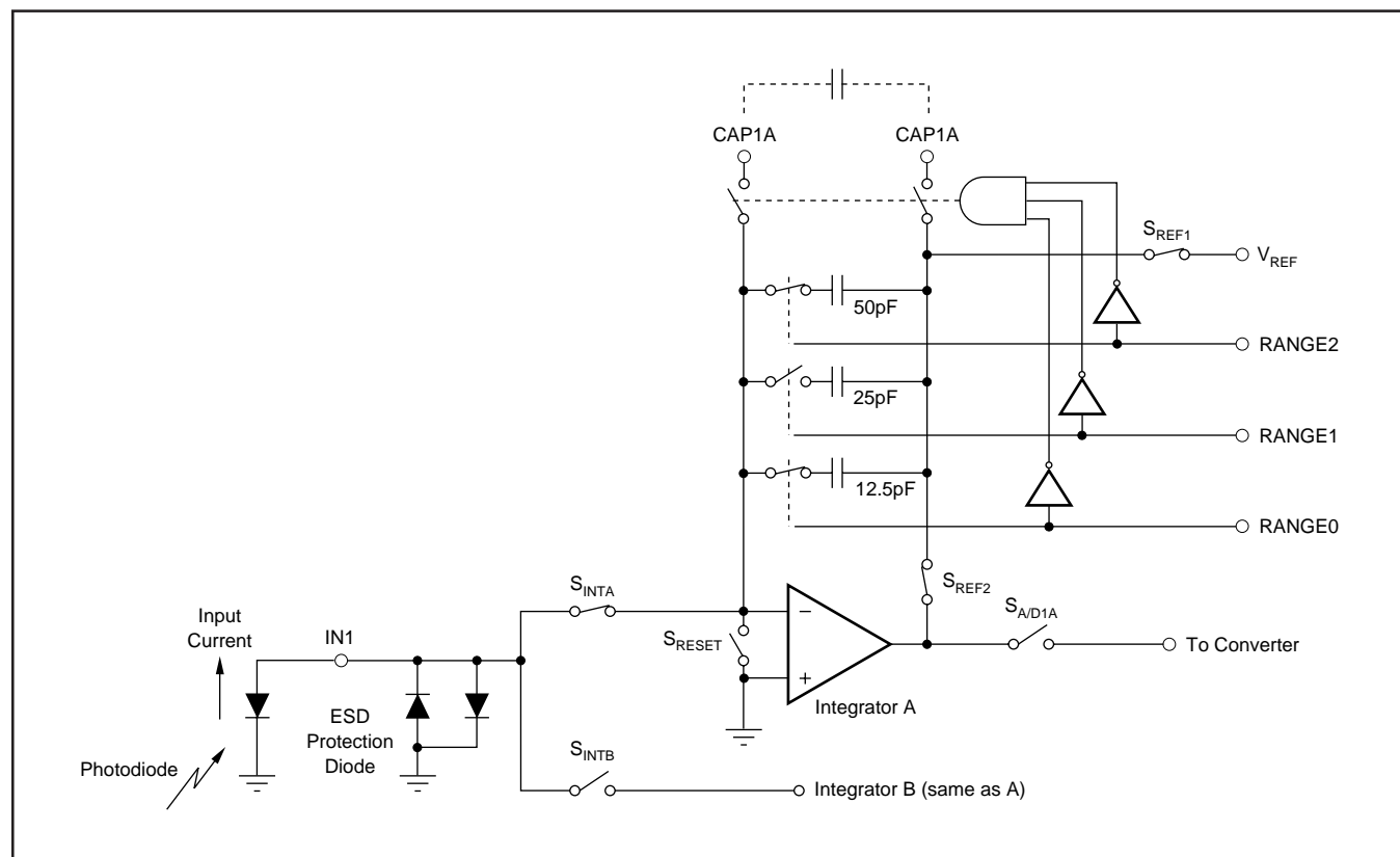
FIGURE 3. Basic Integrator Configuration for Input 1 Shown with a 250pC ( C_F = 62.5 pF) Input Range.
