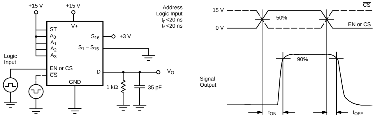
FIGURE 2. EN, CS, \overline{CS} , Turn On/Off Time
