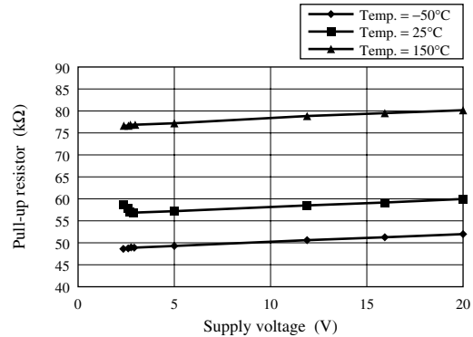
Pull-up resistor — Supply voltage
