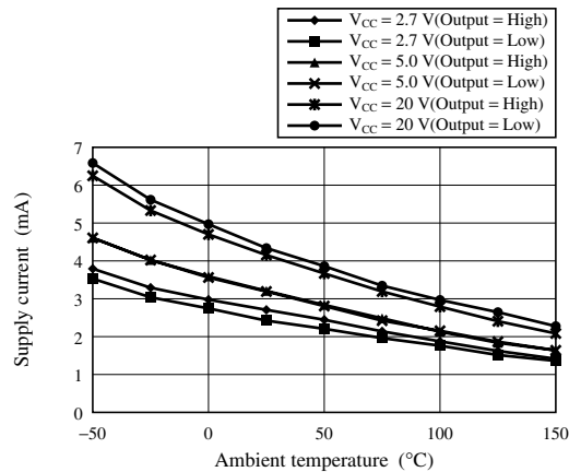
Supply current — Ambient temperature
