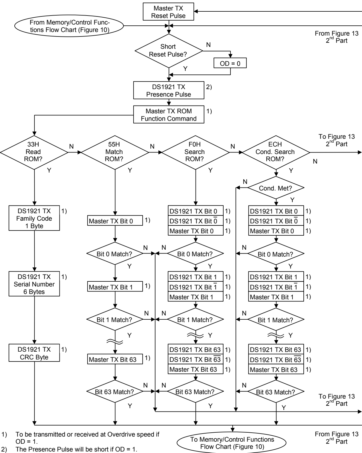
Figure 13-1. ROM FUNCTIONS FLOW CHART
