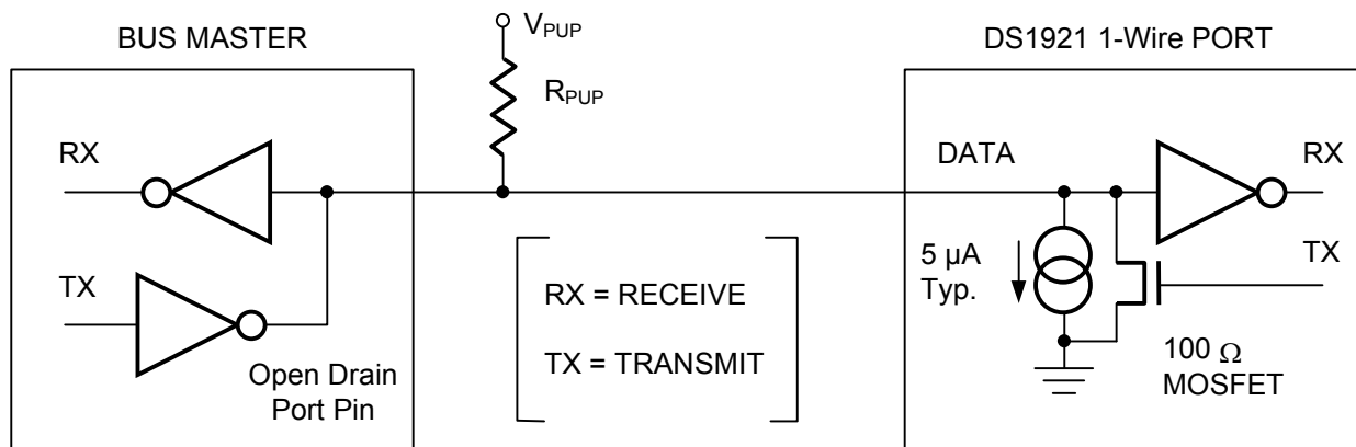
Figure 12. HARDWARE CONFIGURATION
