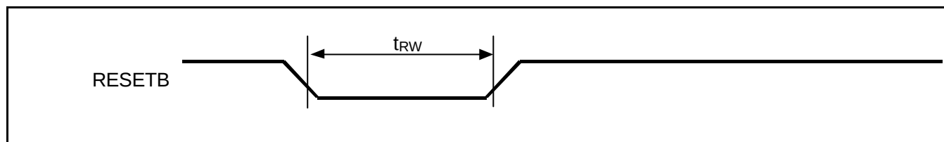
Figure 41. Reset Input Timing
