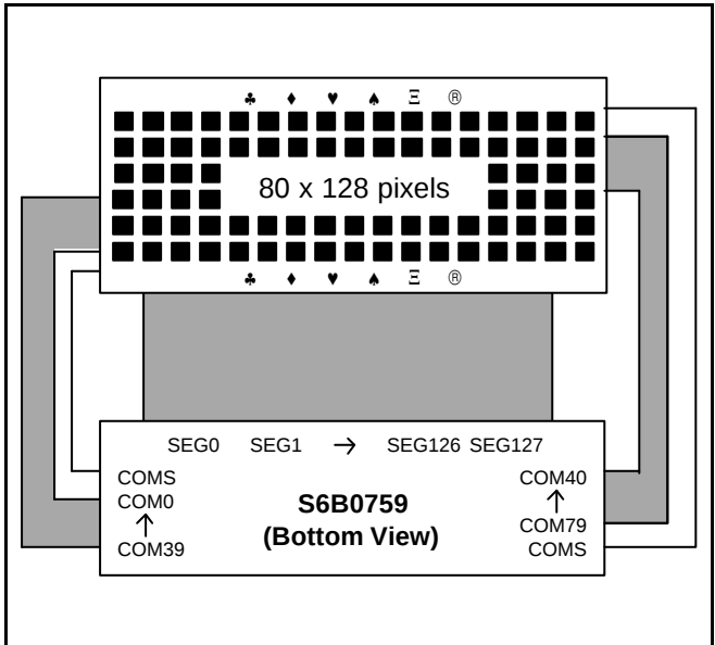
Figure 53. SHL = 1, ADC = 0
