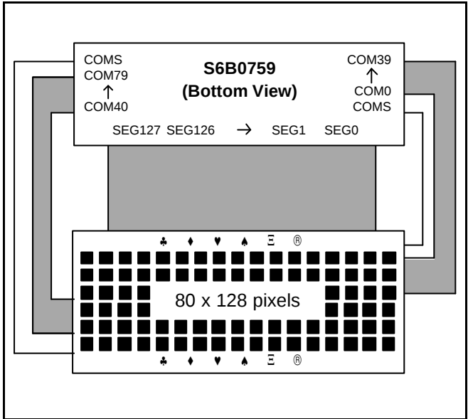
Figure 51. SHL = 0, ADC = 1
