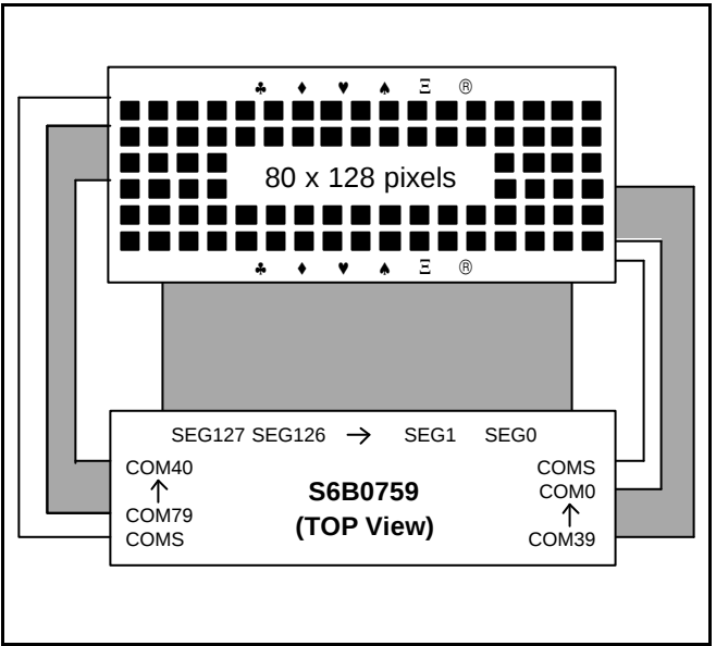
Figure 54. SHL = 1, ADC = 1
