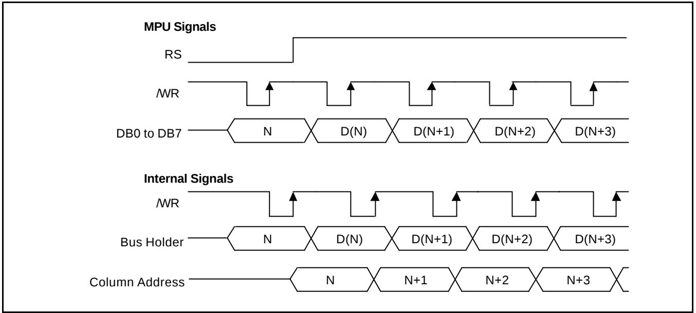
Figure 7. Write Timing
