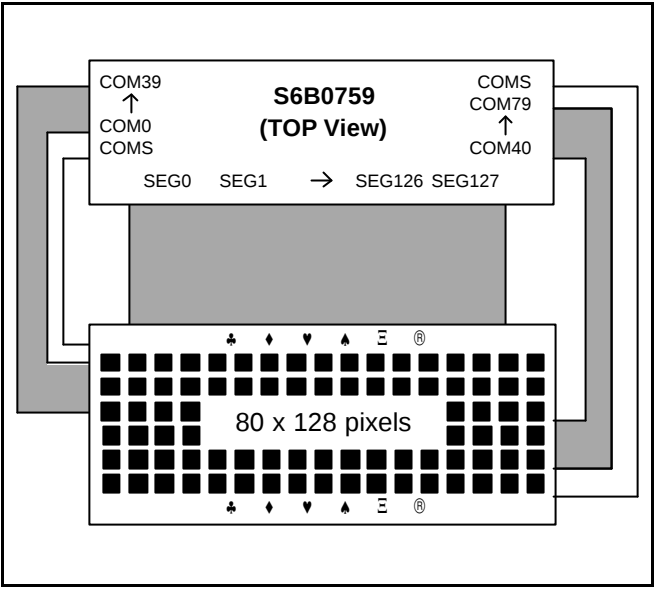
Figure 52. SHL = 0, ADC = 0
