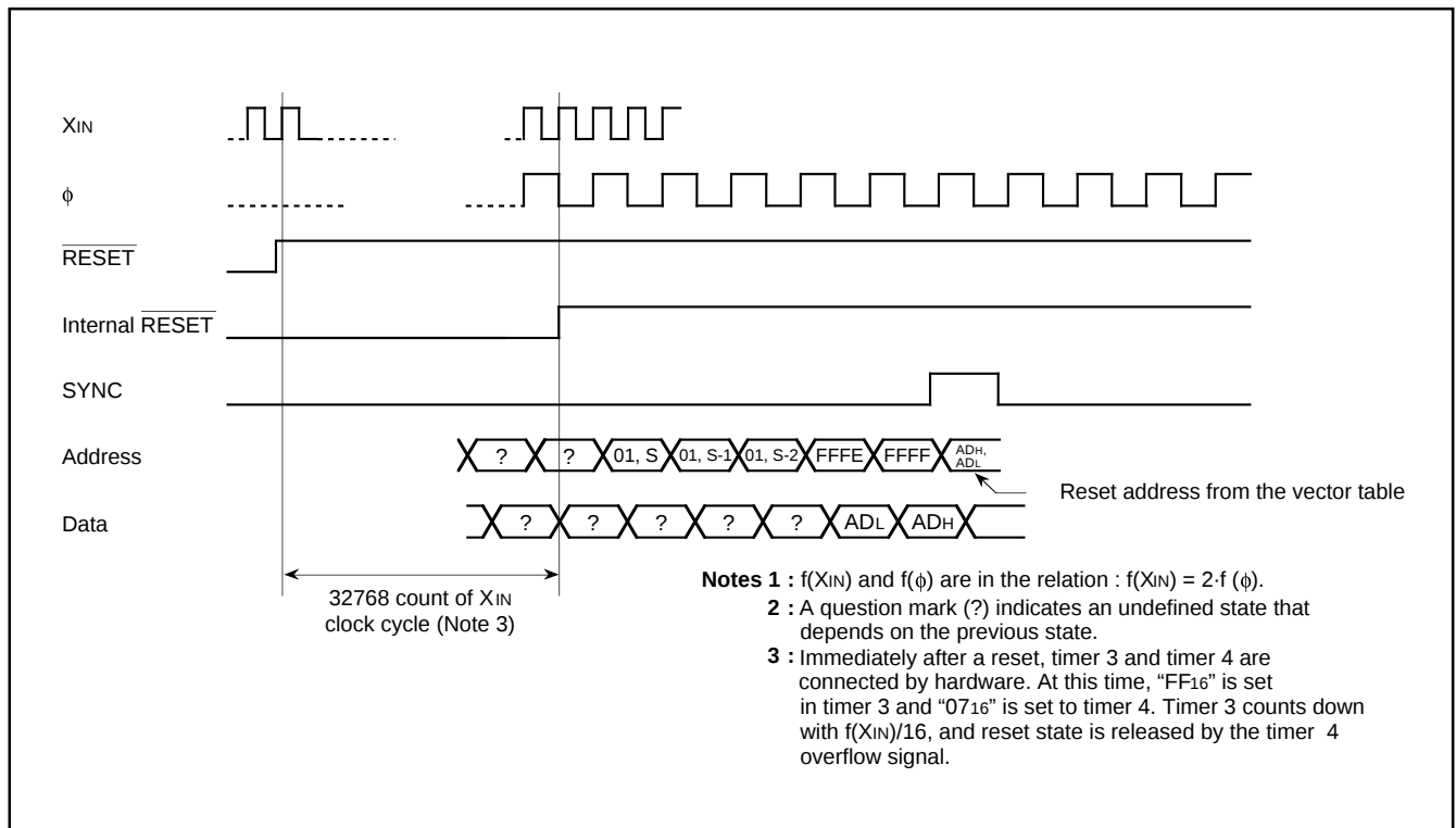
Fig. 77. Reset Sequence
