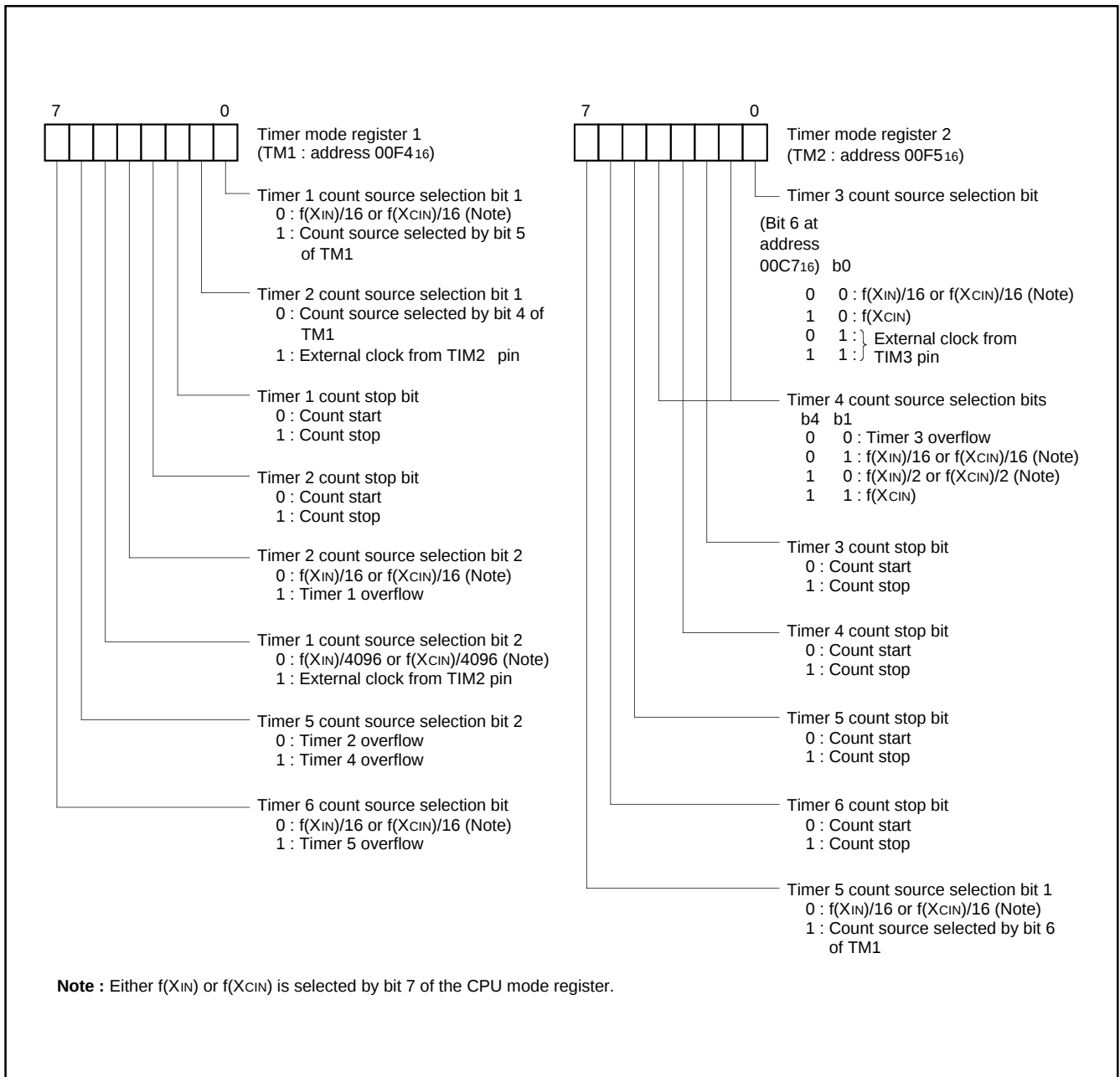
Fig. 11. Timer-related Registers
