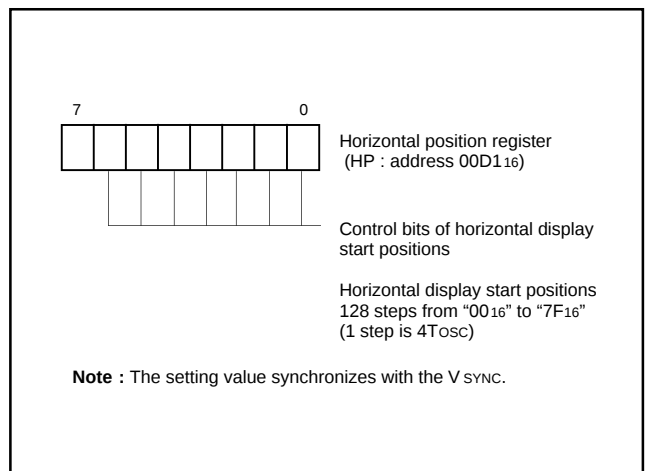
Fig. 52. Horizontal Position Register
