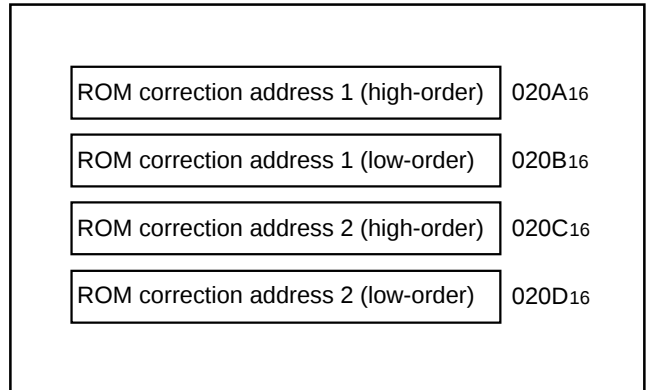
Fig. 74. ROM Correction Address Registers
