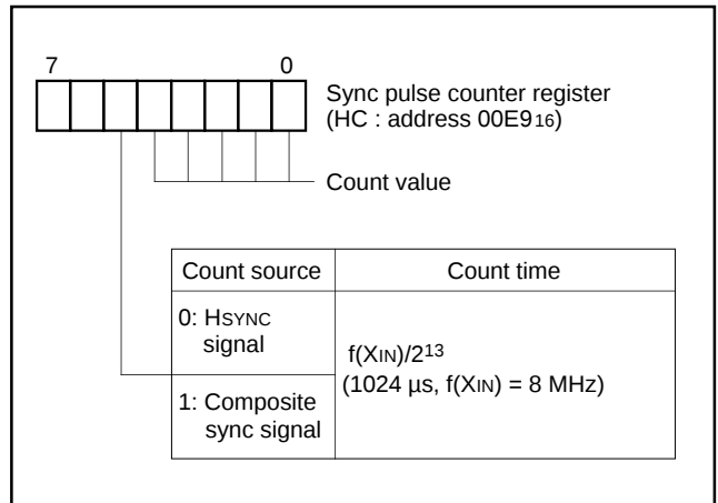
Fig. 32. Sync Pulse Counter Register
