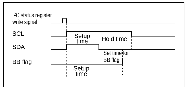
Fig. 41. START Condition Generation Timing Diagram
