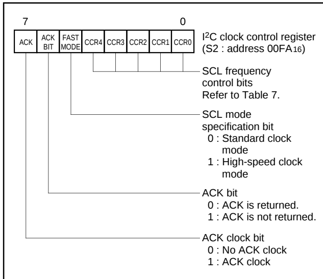
Fig. 36. I²C Clock Control Register
