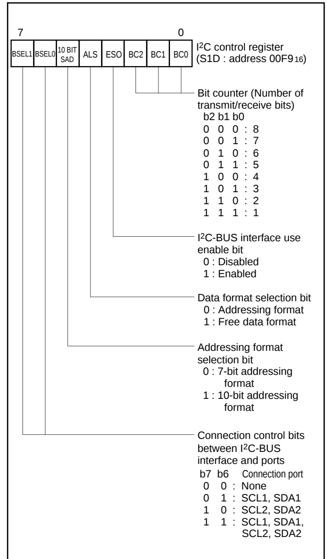
Fig. 38. I²C Control Register
