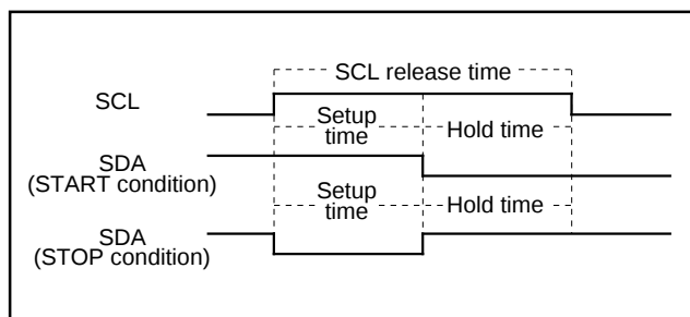
Fig. 43. START Condition/STOP Condition Detect Timing Diagram
