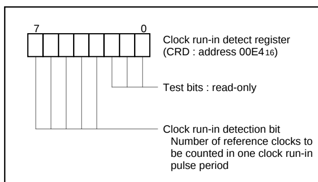
Fig. 30. Clock Run-in Detect Register
