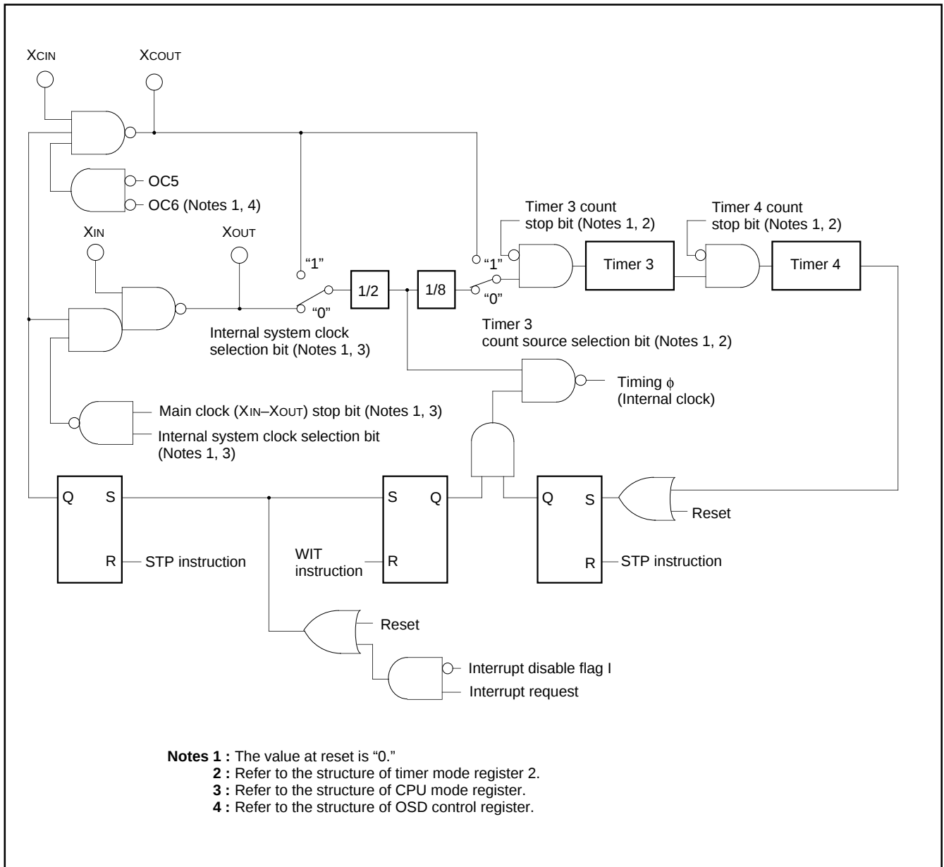
Fig. 80. Clock Generating Circuit Block Diagram
