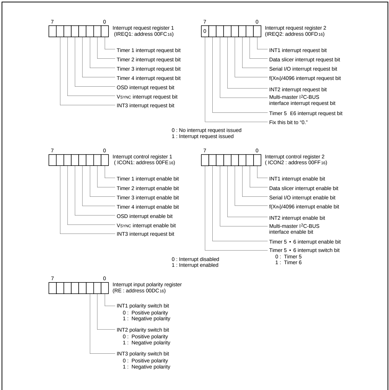
Fig. 9. Interrupt-related Registers
