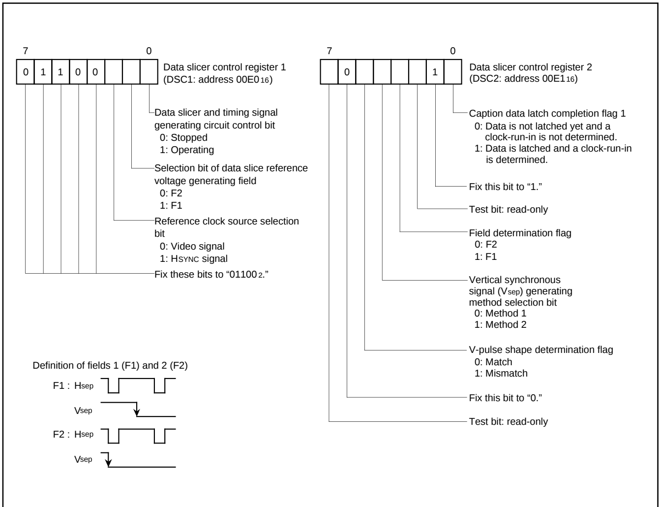
Fig. 25. Data Slicer Control Registers
