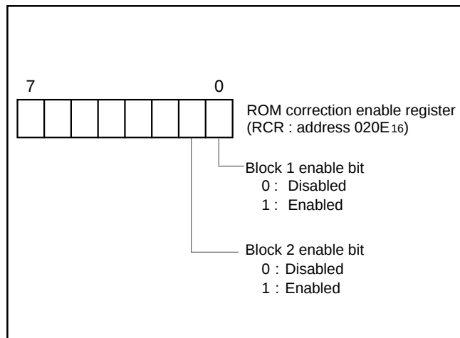
Fig. 75. ROM Correction Enable Register
