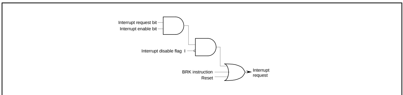
Fig. 10. Interrupt Control
