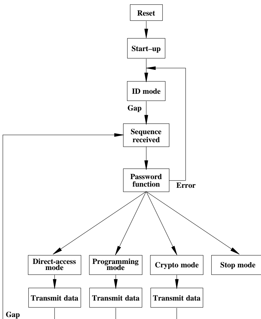
Figure 2. State diagram of the e5561 (overview)
