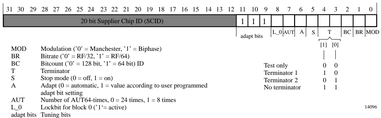
Figure 8. Configuration data in block 0
