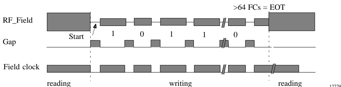
Figure 14. Signals to the transponder during writing
