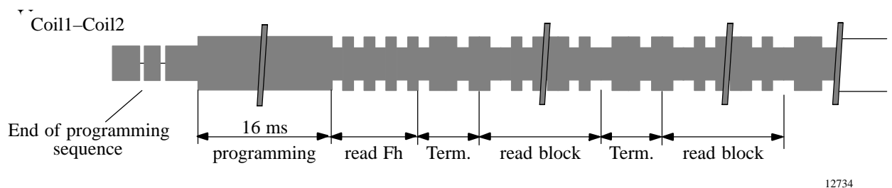
Figure 20. Coil voltage in programming mode
