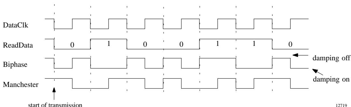
Figure 4. Types of modulation
