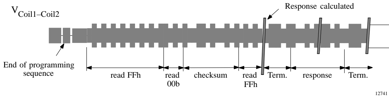
Figure 28. Coil voltage in crypto mode
