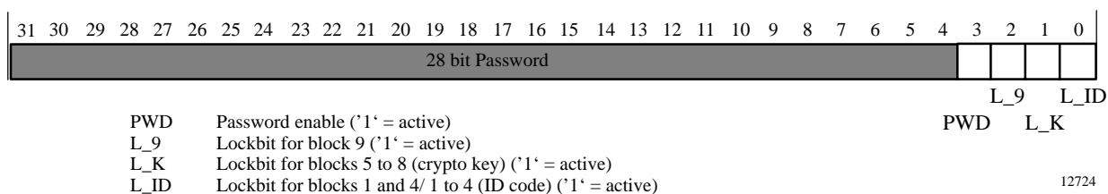
Figure 9. Customer configuration data in block 9
