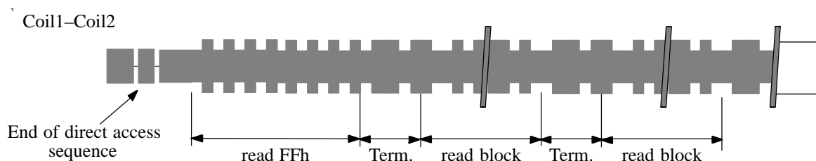
Figure 22. Direct-access mode datastream
