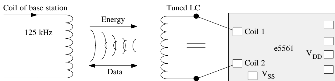
Figure 6. Application circuit
