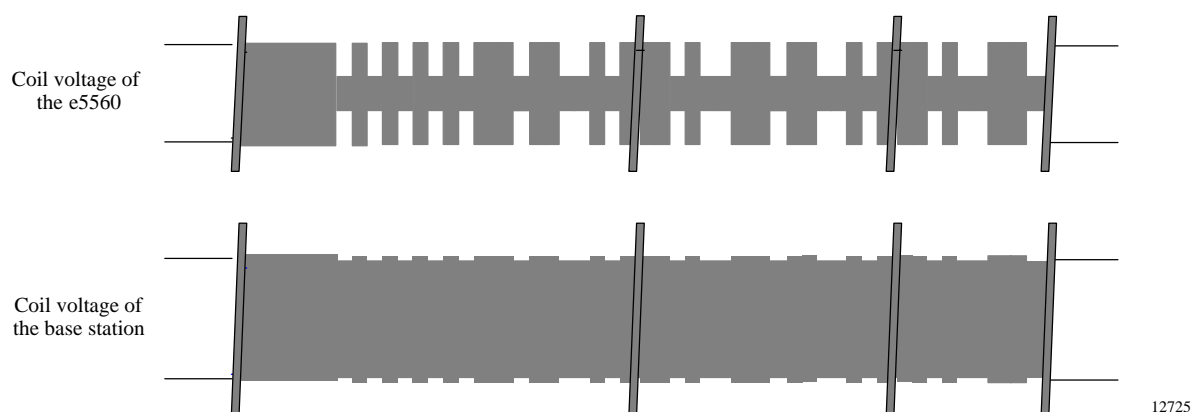
Figure 10. Signals from the transponder during reading
