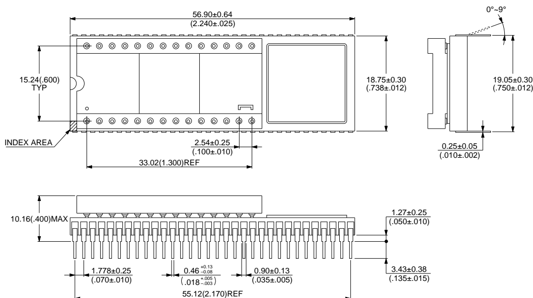
64-pin Ceramic MDIP (MDP-64C-P02)
