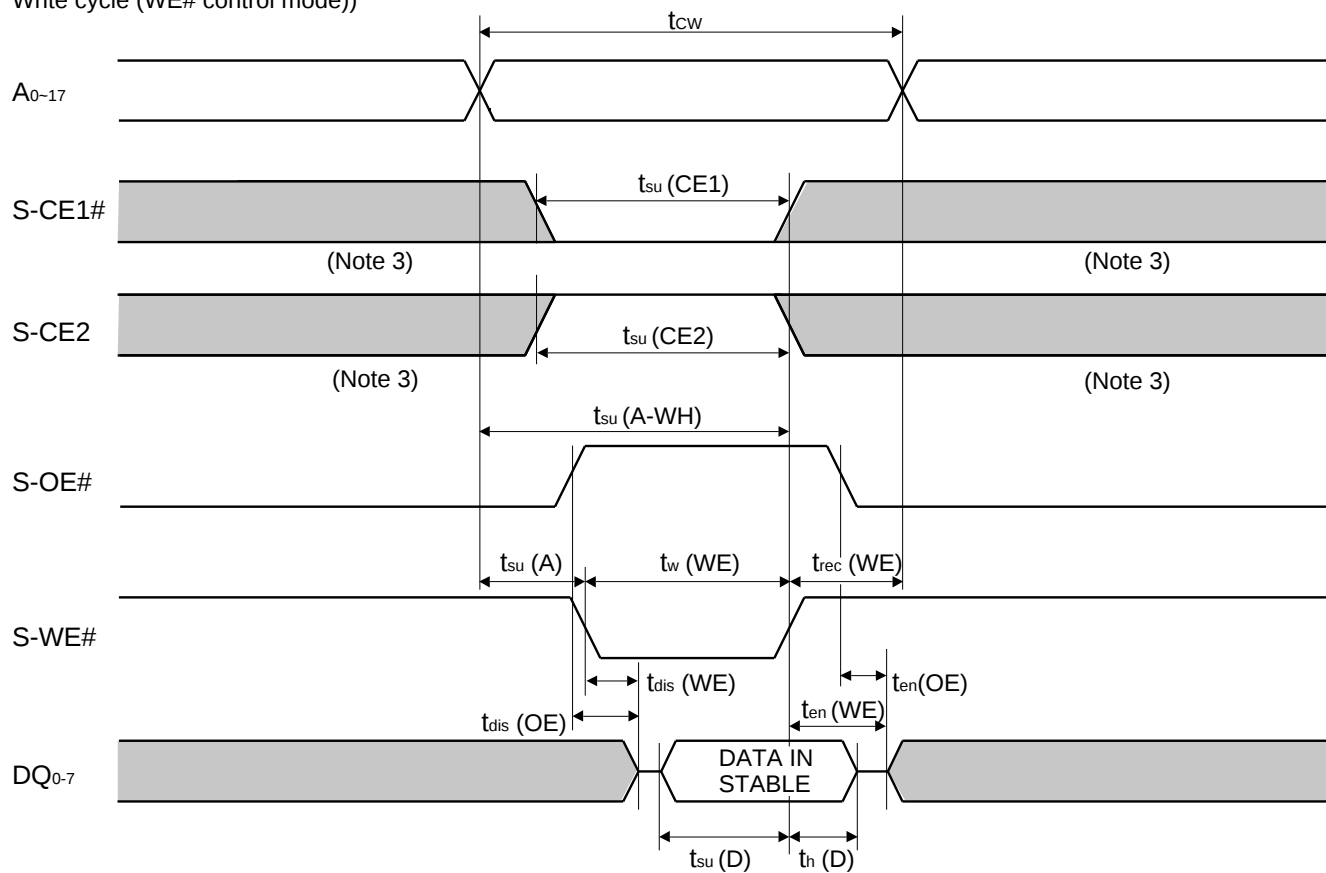
Write cycle (WE# control mode)
