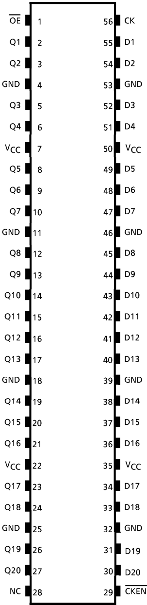
(TOP VIEW)
