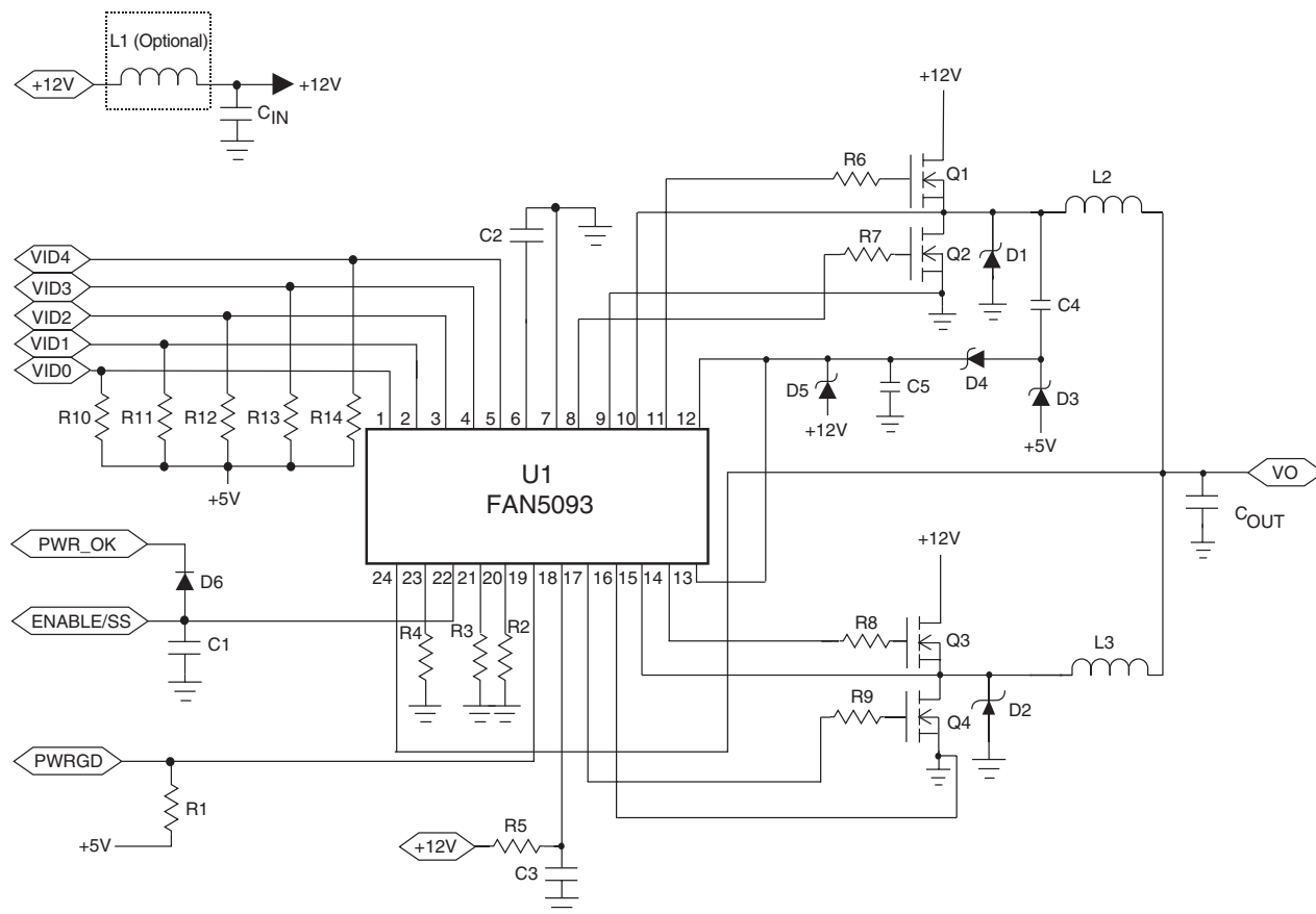
Figure 3. Application Circuit for 35A High-Frequency Application (1MHz each phase)
