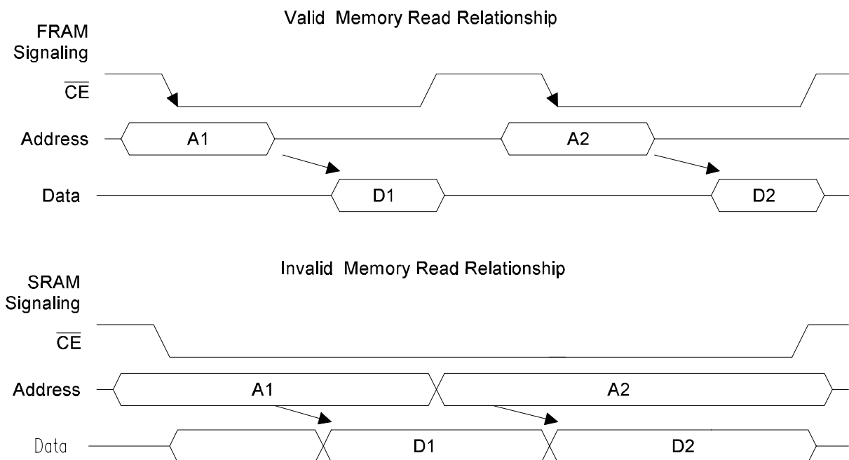
Figure 2. Memory Address and \overline{\text{CE}} Relationships
