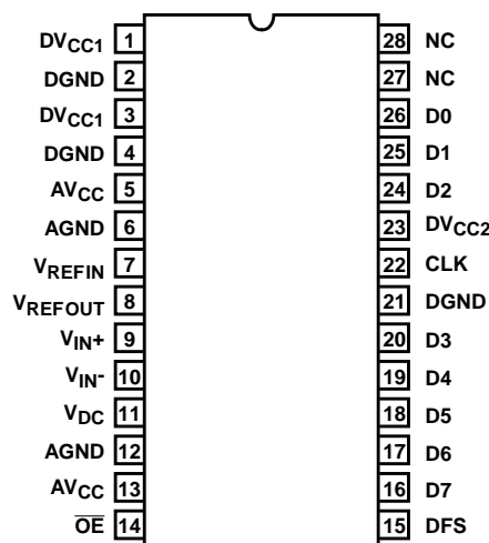
HI5667 (SOIC, SSOP) TOP VIEW
