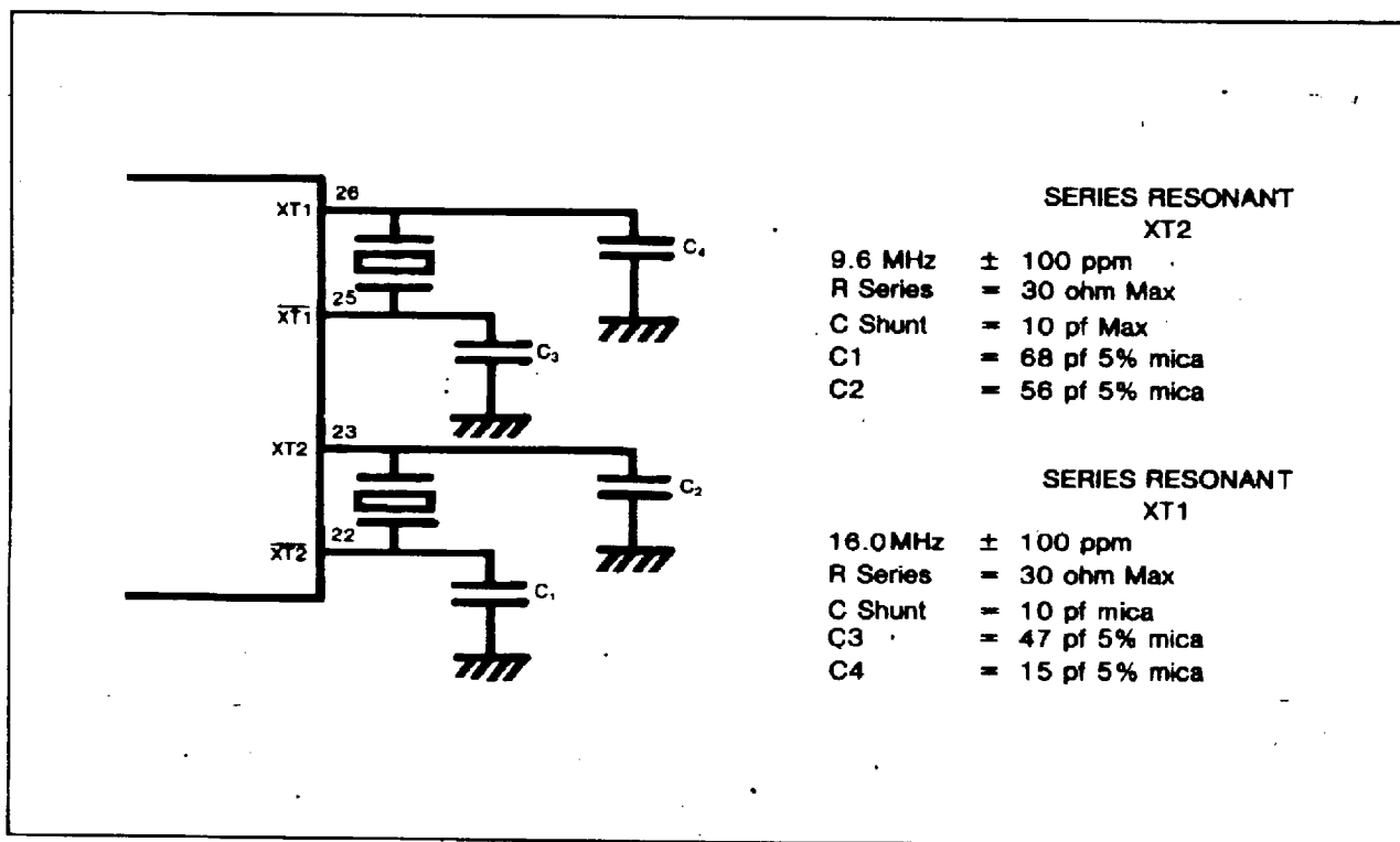
Fig 6. XTAL Oscillator circuits for the 44 pin PLCC
