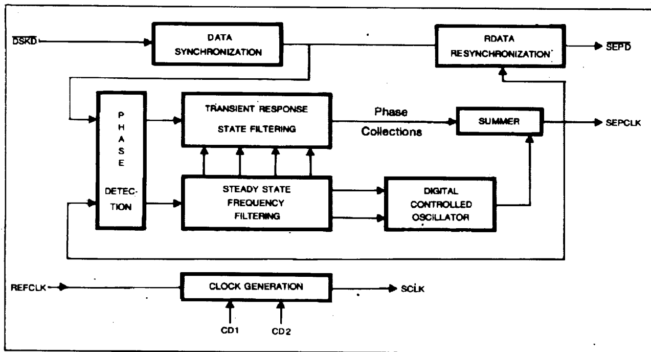
Fig. 5. DPLL Simplified BLOCK DIAGRAM
