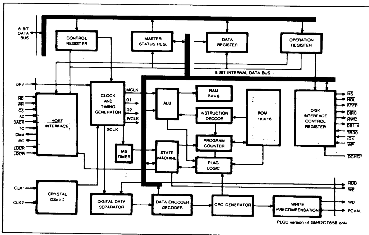
Fig 1. GM82C765B Internal Block Diagram
