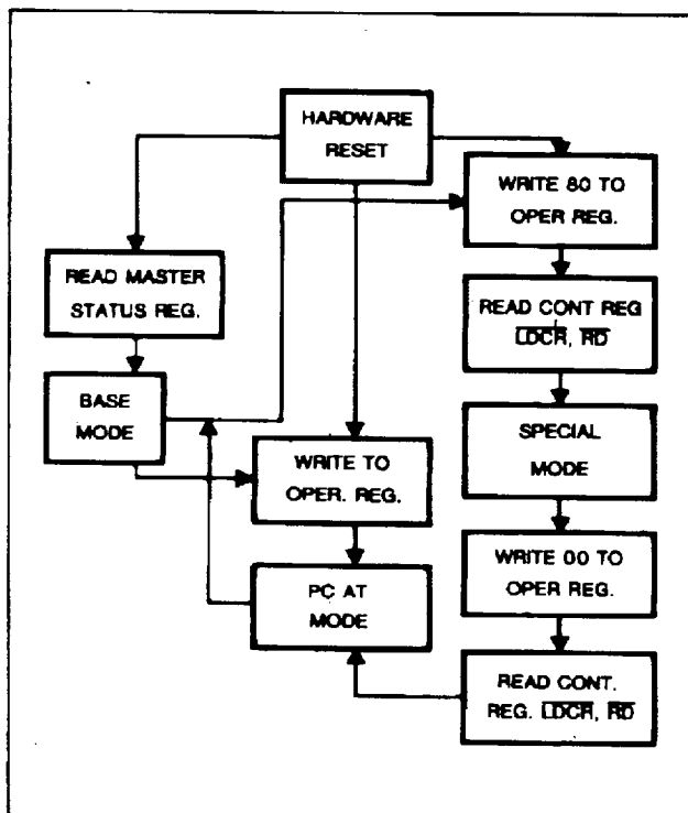
Fig. 3. Flow Diagram Depicting Relationship of Base, Special, and PC AT modes.
