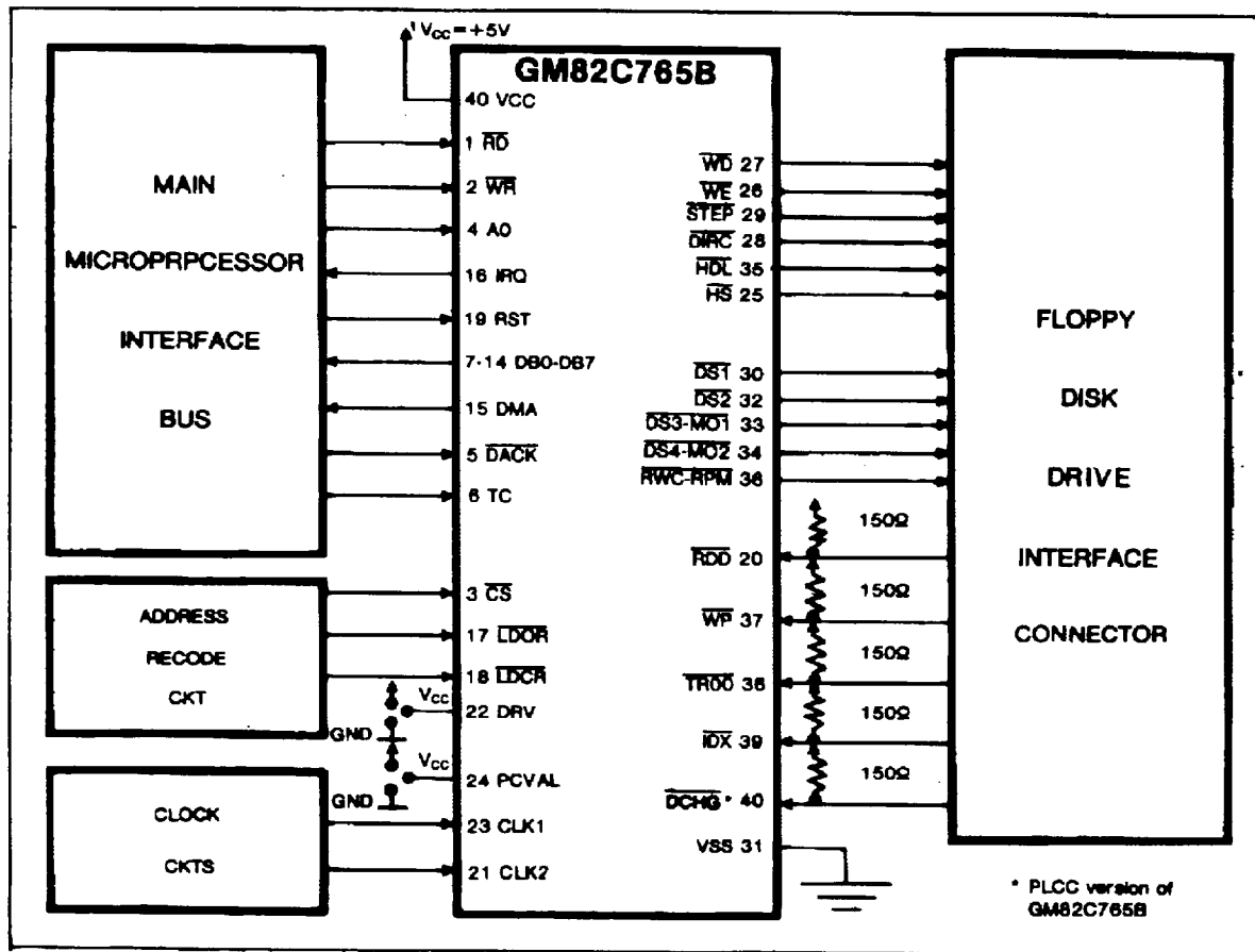
Fig. 2. TYPICAL GM 82C765B APPLICATION SYSTEM.
