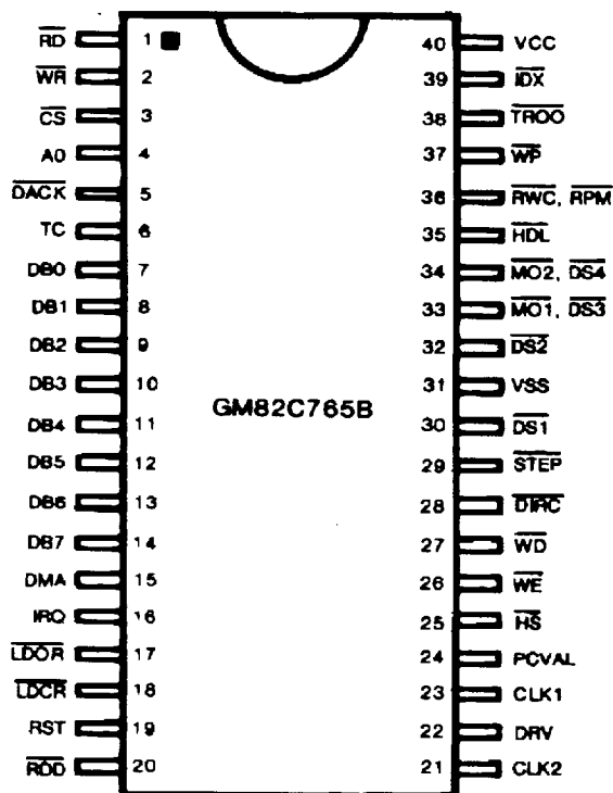
40 PIN DIP
