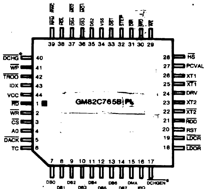
44 PIN PLCC
