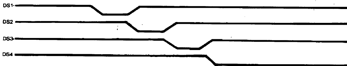
Fig. 4. Drive select polling timing
