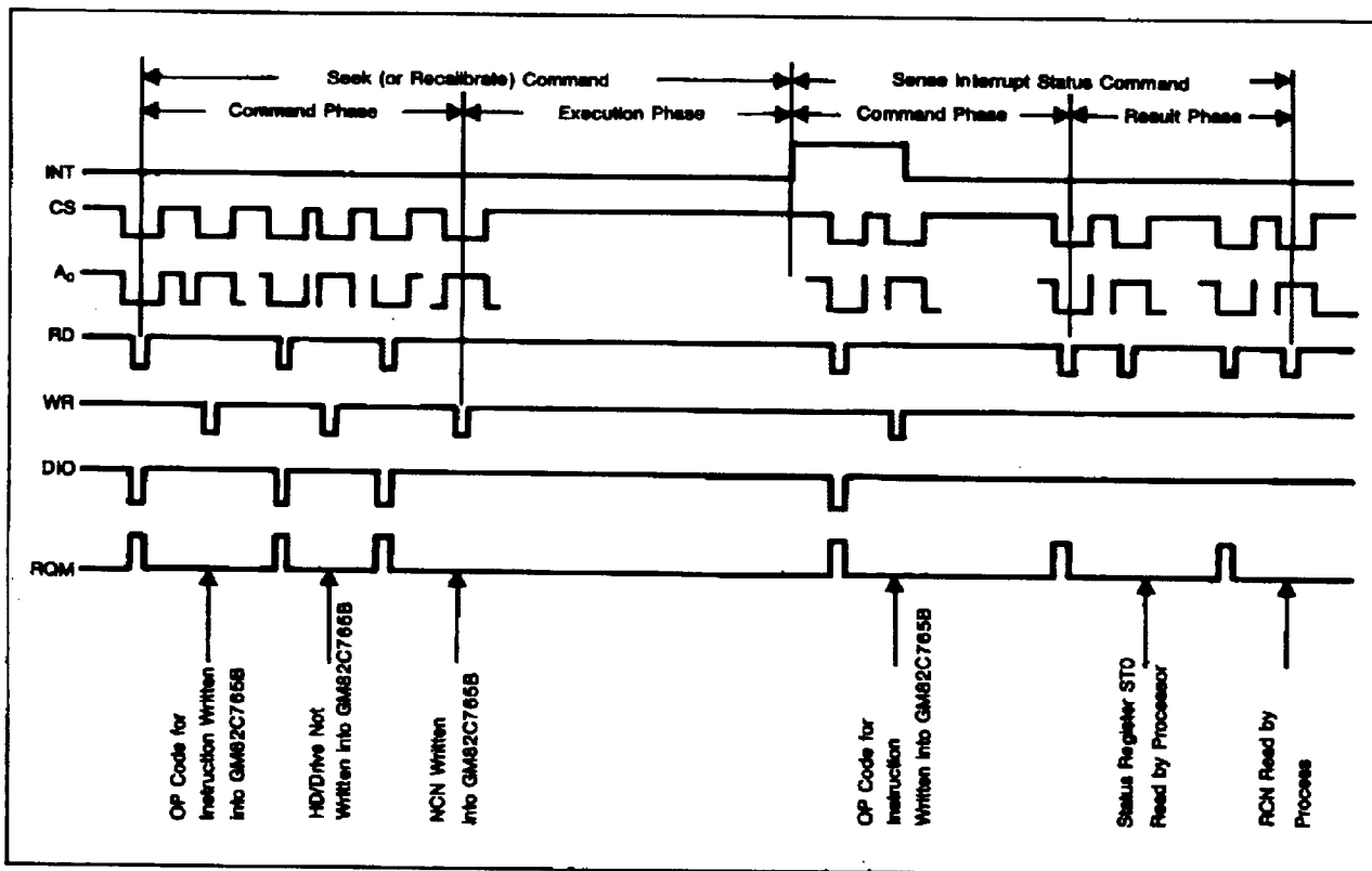
Fig. 7. Seek, Recalibrate and Sense Interrupt Relationship
