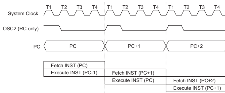
Execution Flow
