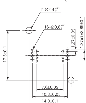
SOP IC51-0162-658 (16 Pins)
