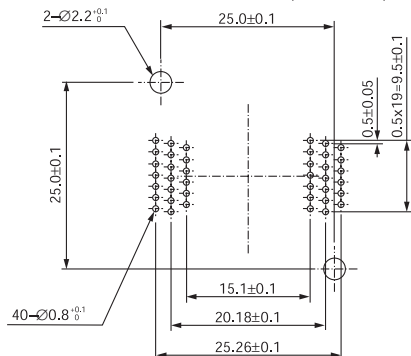
TSOP IC51-0402-1174-1 (40 Pins)
