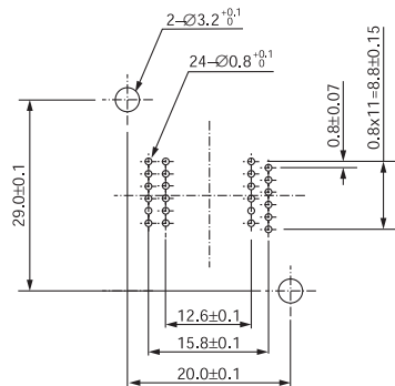
SOP IC51-0242-577 (24 Pins)
