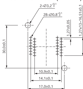
SOP IC51-0282-986 (28 Pins)
