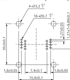
SOP IC51-0162-658 (16 Pins)
