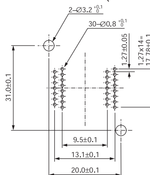
SOP IC51-0302-1017 (30 Pins)
