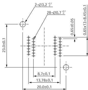
SSOP IC51-755.KS-13330 (28 Pins)
