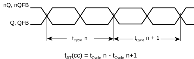
CYCLE-TO-CYCLE JITTER
