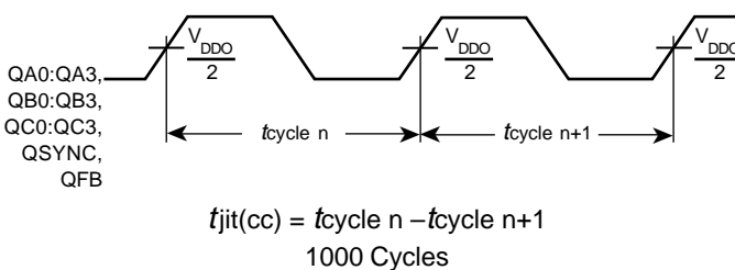
CYCLE-TO-CYCLE JITTER
