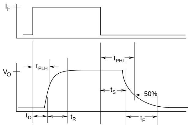
Figure 1. Switching waveform
