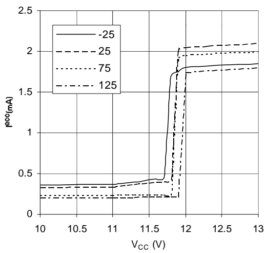
Chart 29. I_{QCC} vs V_{CC} vs Temp V_{CCUV+}
