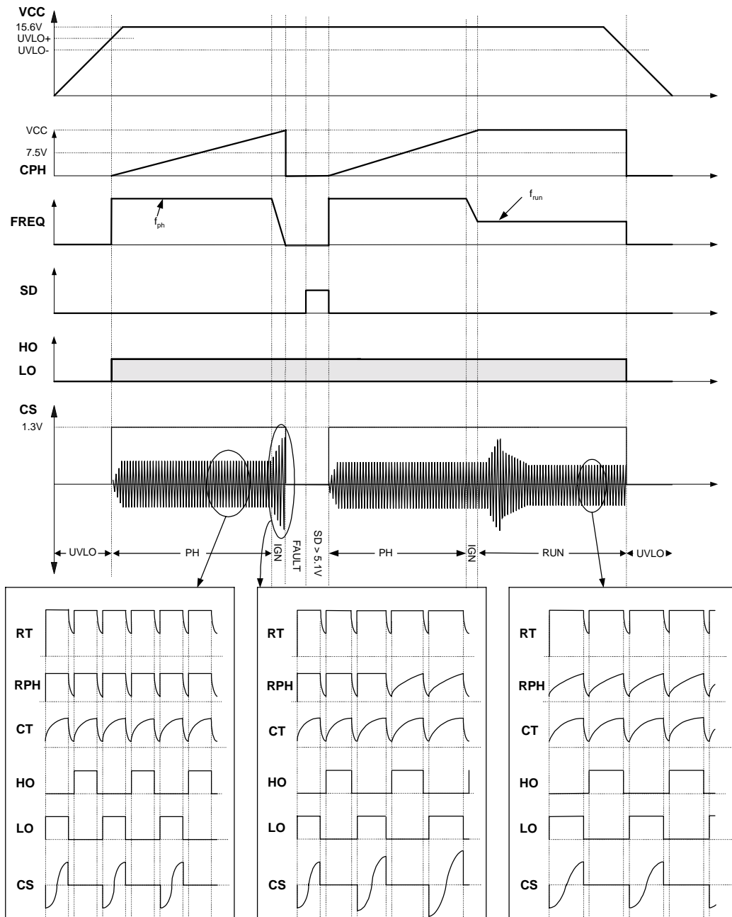
BALLAST TIMING DIAGRAMS FAULT CONDITION
