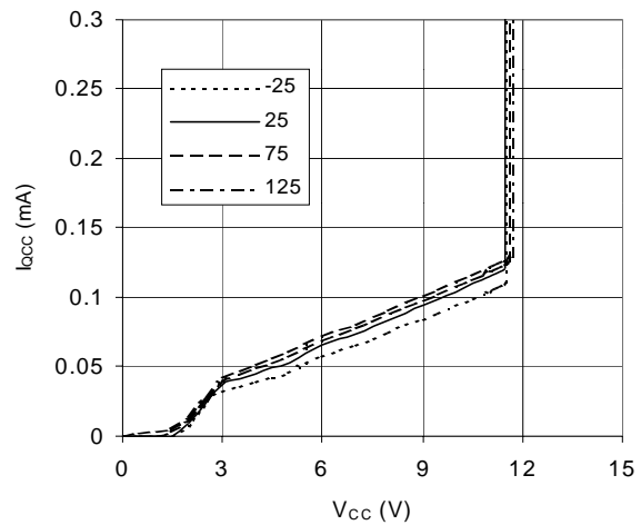
Graph 28. I_{QCC} vs V_{CC} vs Temp Micropower Startup Mode
