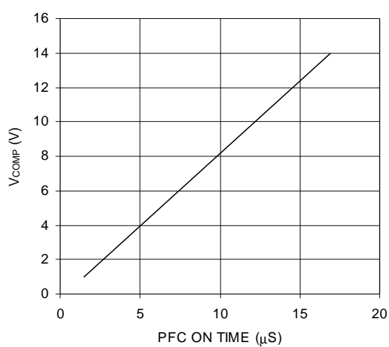
Graph 24: VCOMP vs PFC ON TIME
