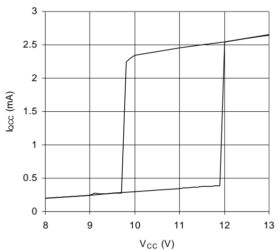
Graph 23: Iacc vs Vcc UVLO Hysteresis
