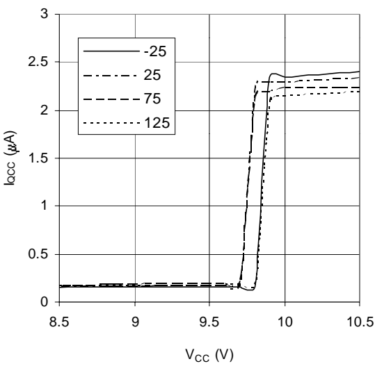
Chart 30. I_{QCC} vs V_{CC} vs Temp V_{CCUV-}
