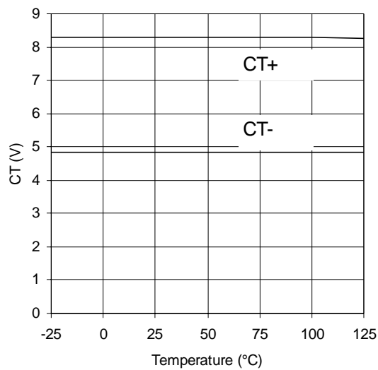
Graph 3: CT+, CT- vs TEMP
