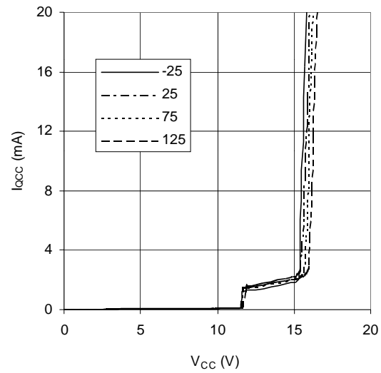
Graph 26. I_{QCC} vs V_{CC} vs Temp
