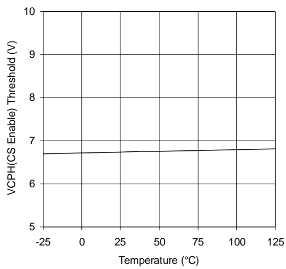
Graph 22: VCPH (CS Enable) Threshold vs TEMP
