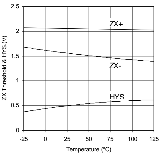
Graph 8: ZX+, ZX- vs TEMP
