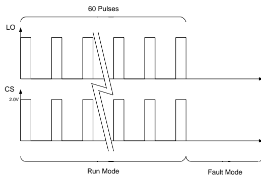
Figure 5: CS & LO Waveforms
