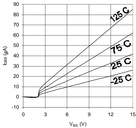
Graph 25. I_{QBS}(1) vs V_{CC} vs Temp
