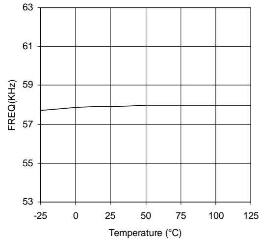
Graph 14: Frequency vs TEMP
