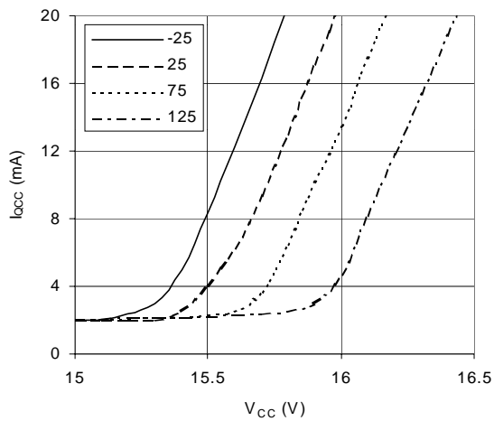
Graph 27. I_{QCC} vs V_{CC} vs Temp Internal Zener Diode Curve
