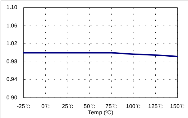
Figure 15. Burst Mode Sync. High Threshold Voltage
