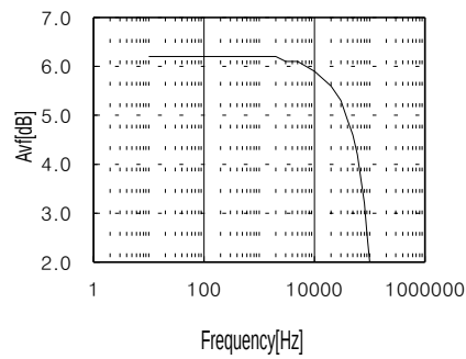
Figure 8. Frequency vs. Avf
