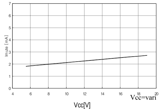
Figure 2. VCC vs. Imute
