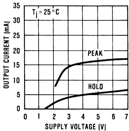
Output Current vs Supply Voltage
