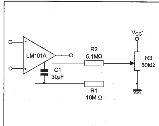
FEEDFORWARD COMPENSATION
