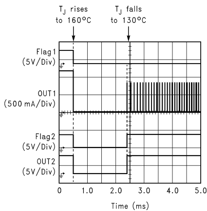
FIGURE 4. Thermal Shutdown Characteristics when Both First-Stage and Second-Stage Thermal-Shutdown Modes are Needed
