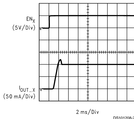
Inrush Current to Downstream Device when LM3544 is Enabled (Note 11)
