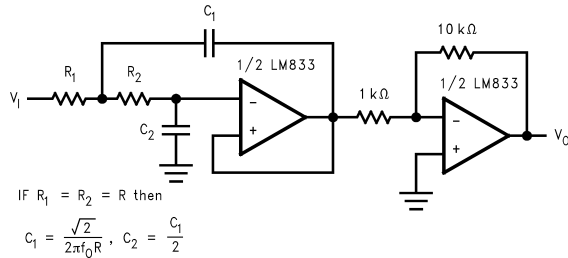
FIGURE 6. Pre-amplifier Stage with Low Pass Filter
