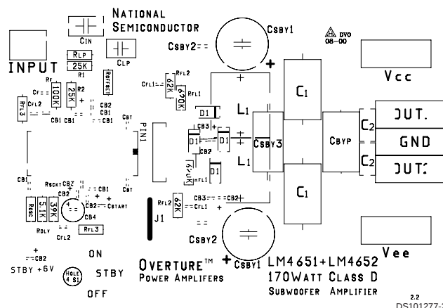
FIGURE 7. Reference PCB silkscreen layer
