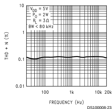
LM4871LD THD+N vs Frequency
