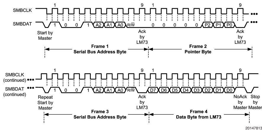
(d) Typical Pointer Set Followed by Immediate Read of a 1-Byte Register.
