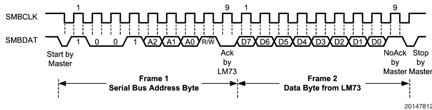
(c) Typical Read from a 1-Byte Register with Preset Pointer
