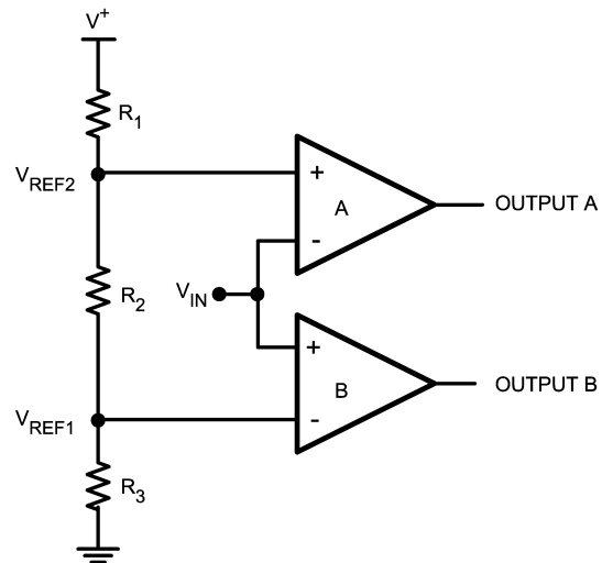
FIGURE 11. Window Detector
