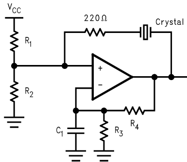
FIGURE 8. Crystal Oscillator
