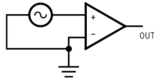
FIGURE 5. Zero Crossing Detector
