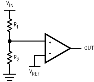
FIGURE 7. Threshold Detector
