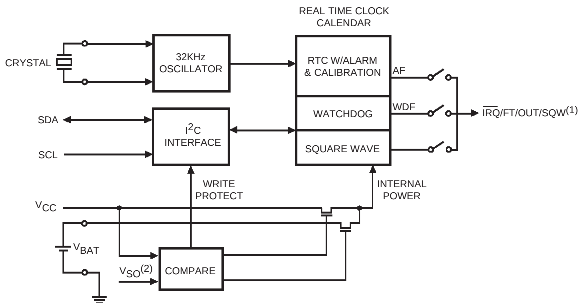
Figure 6. Block Diagram
