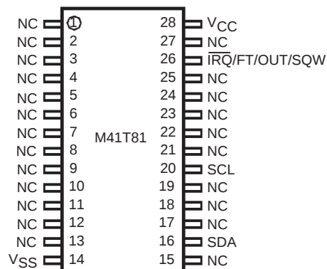
Figure 5. 28-pin SOIC Connections
