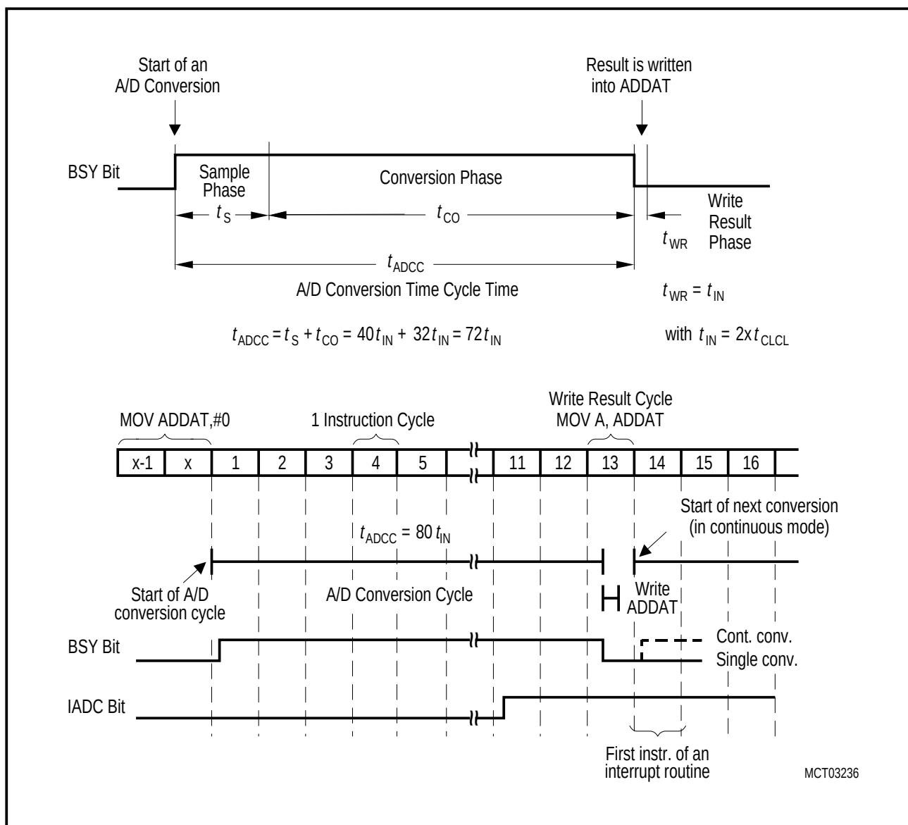
Figure 6-33 A/D Conversion Timing
