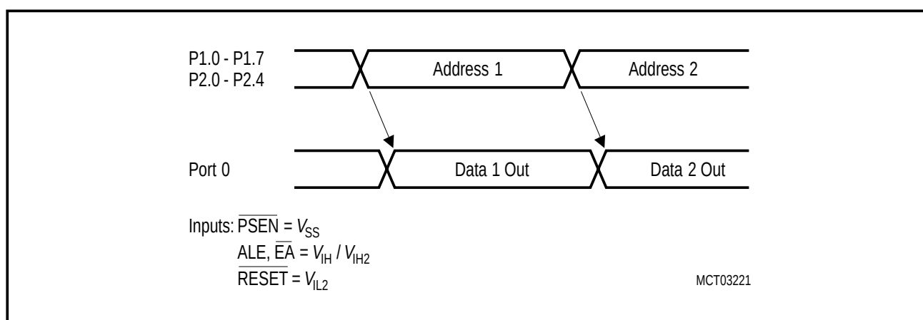
Figure 4-3 ROM Verification Mode 1
