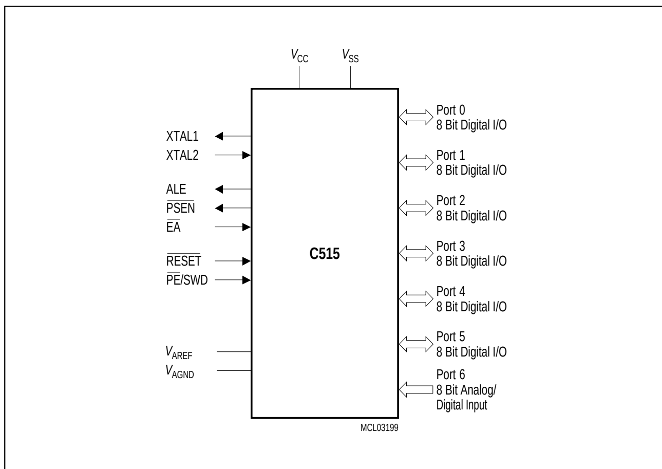
Figure 1-2 Logic Symbol
