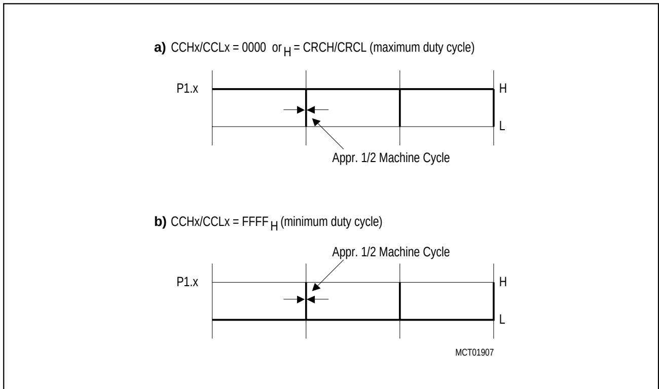
Figure 6-18 Modulation Range of a PWM Signal, generated with a Timer 2/CCx Register Combination in Compare Mode 0*
