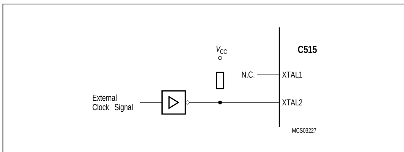
Figure 5-5 External Clock Source
