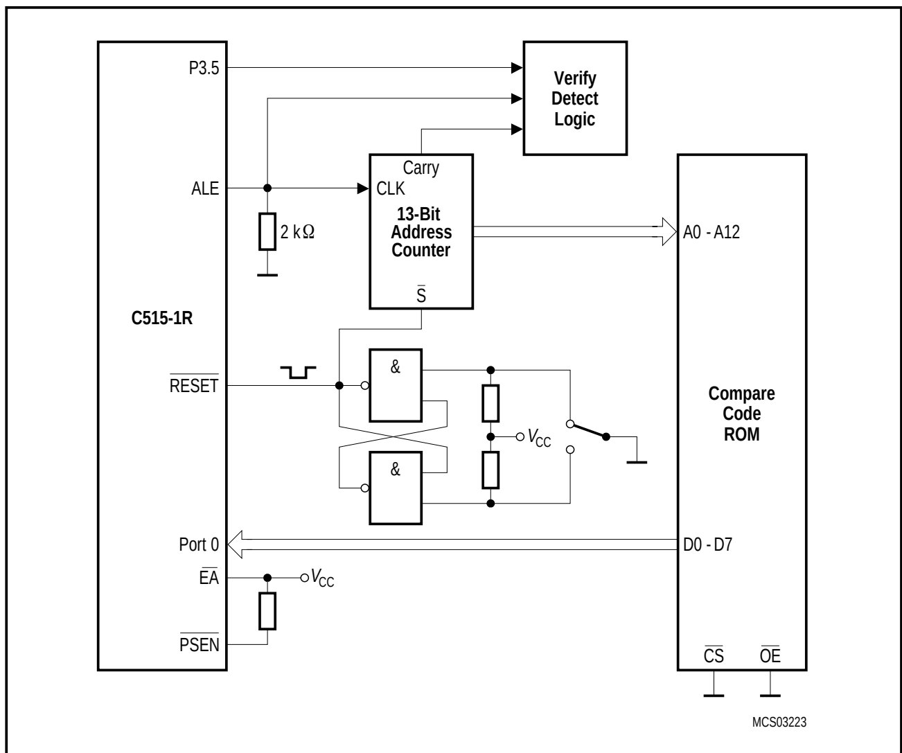
Figure 4-5 ROM Verification Mode 2 - External Circuitry Example
